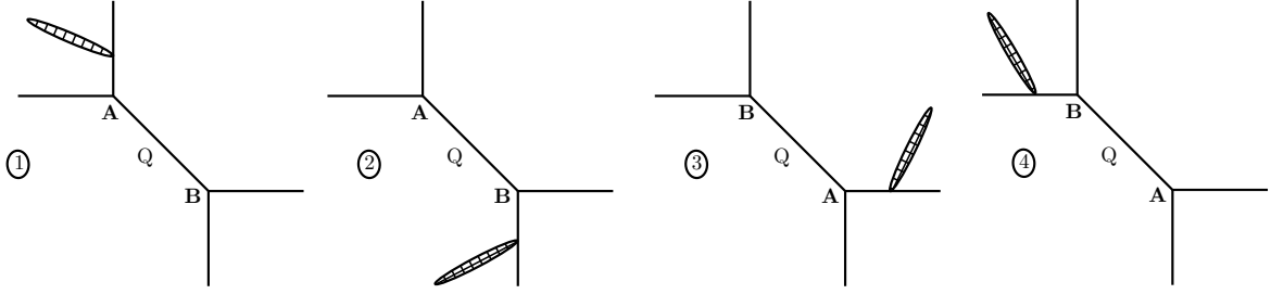
Figure 5. Toric diagram for resolved conifold.
