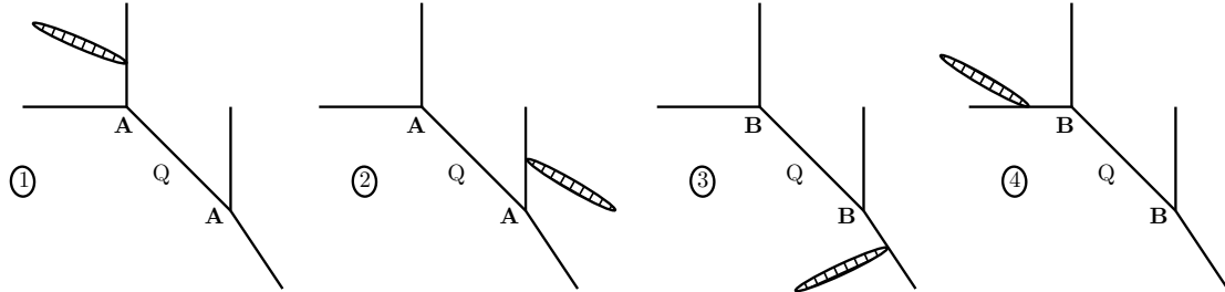
Figure 15. Branes attached to various legs of a diagram for the resolution of \mathbb{C}^3/\mathbb{Z}_2 .
