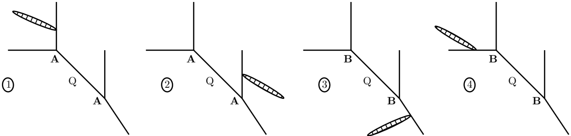
Figure 6. Toric diagram for a resolution of \mathbb{C}^3/\mathbb{Z}_2 .
