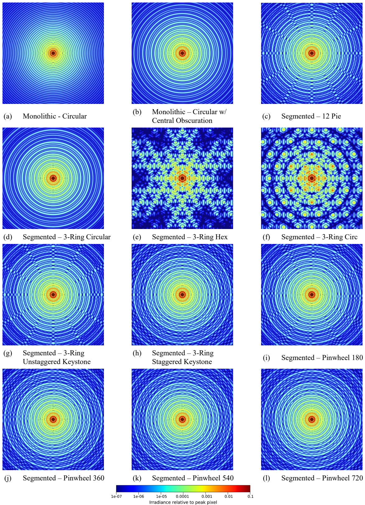
Figure 5: Illustration PSFs within 1 arcsec field of view for each of the pupils listed in Figure 4, calculated at wavelength 1\mu\text{m} . The PSFs are all in log scale with color bar at the bottom indicated the value. (Please, watch the Media 1 for the PSF variations.)
