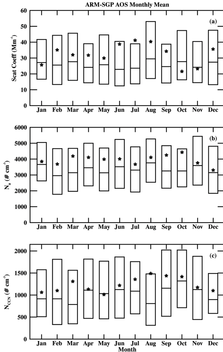
Figure 1. 2008-2016 monthly mean (asterisk) and median Aerosol Observation System (AOS) (a) scattering coefficient, (b) aerosol number concentration ( N_a ), and (c) cloud condensation nuclei number concentration ( N_{CCN} ). The interquartile range (IQR) is added to show the spread of the AOS measurements. Note the seasonality of the dataset which is more positively skewed during the summer and autumn (JJASO) months with a second maximum from late winter through the spring (FMAM).
