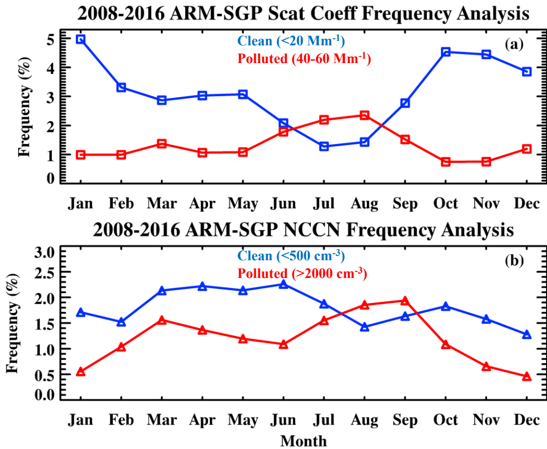
Figure 3. Frequency analysis of the mean monthly Aerosol Observation System (AOS) (a) scattering coefficient and (b) number concentration of CCN. Note that clean continental conditions are more frequent for most of the year except during the summer months.
