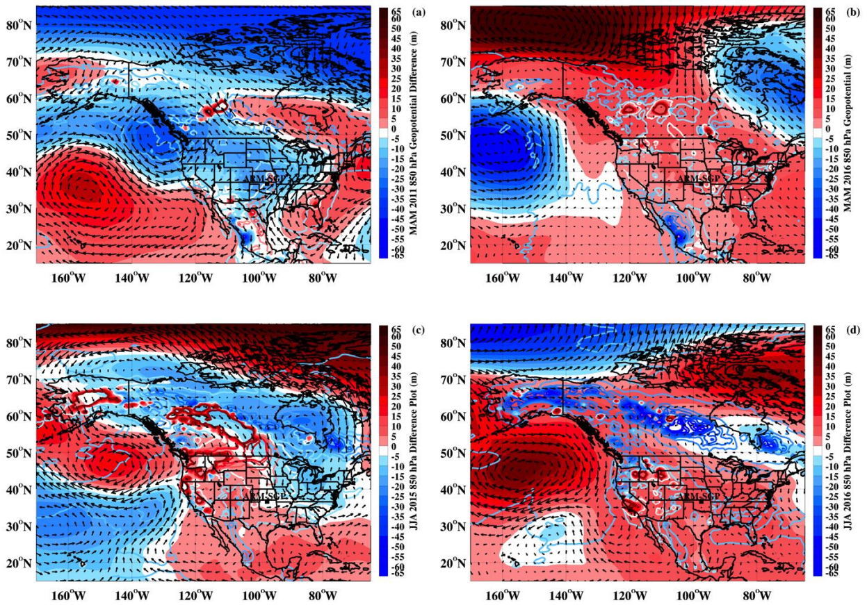
Figure 5. MERRA-2 domain isobaric height anomalies for (a) Spring 2011, (b) Spring 2016, (c) Summer 2015, and (d) Summer 2016. The anomalies are derived by subtracting the 1981-2016 climate domain mean. The red (blue) regions denote positive (negative) height anomalies in which wind motions are anticyclonic (cyclonic) as given by the black arrows. The red (blue) colored line contours denote positive (negative) anomalous MERRA-2 carbonaceous concentrations derived from wildfire activity. Wind data are taken from the NOAA ESRL data repository ( https://www.esrl.noaa.gov/psd/data/composites/day/ ).
