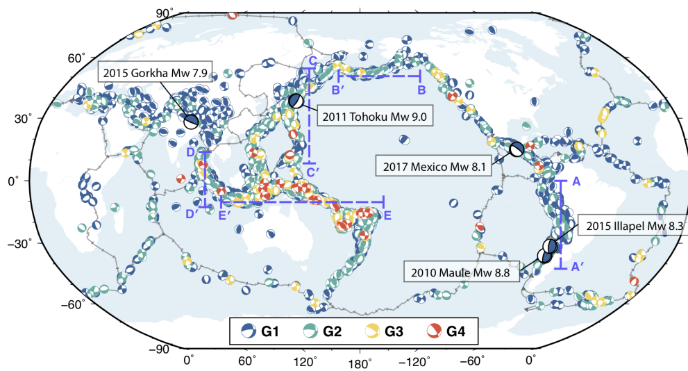
Figure 3. Map of focal mechanisms colored by their group label and overlay of the plate boundaries (gray thin lines). Several recent large megathrust earthquakes are highlighted. Blue dashed lines shown the locations of profiles in Figure 4. Bottom panels show the center STFs in each groups (same as those in Figure 1 (a)) as well as the corresponding schematic rupture propagation.
