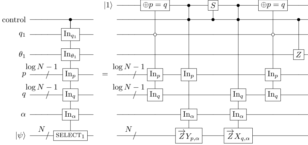
Figure 1: The circuit needed to perform a controlled \text{SELECT}_1 operation. We have omitted the registers this operation does not act upon for simplicity. The unitaries labeled as \vec{Z} A_j apply the operation Z_0 \cdots Z_{j-1} A_j to the target register, depending on the value from the input register, using the technique shown in Figure 9 of [8]. This operation can be achieved using an inequality test, followed by a ranged operation via the technique shown in Figure 8 of [8]. The controlled \text{SELECT}_2 operation is completely equivalent except with different control registers.
