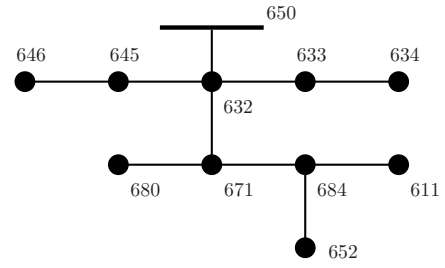
Fig. 1. An 11 bus network revised from IEEE 13 node test feeder. The switch in the original system is assumed to be open so 2 buses are removed.
