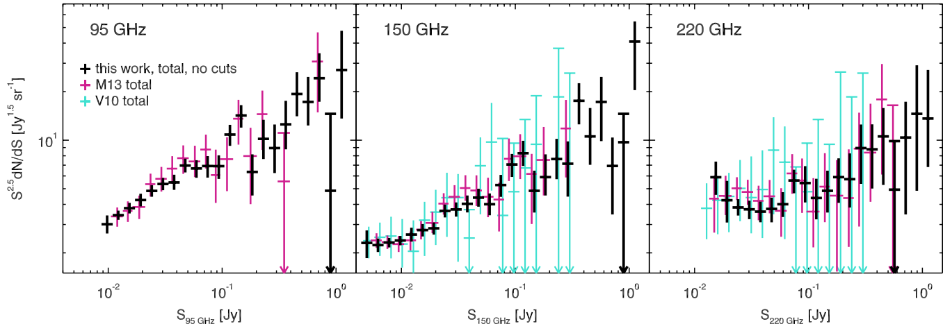
Figure 15. Total source counts (with no cuts applied other than removing sources identified as stars) for the current work, using 2530 square-degrees of the SPT-SZ survey, compared with number counts from M13 (calculated using 771 square degrees of sky area) and V10 (calculated using 87 square degrees of sky area in 150 and 220 GHz only). V10 used a detection threshold of 3\sigma , whereas M13 and the current work use 4.5\sigma to increase the purity of the sample, which resulted in V10 probing a slightly lower flux range than M13 and the current work at 220 GHz.
