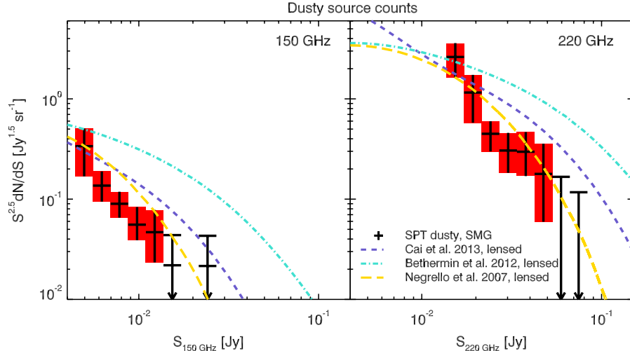
Figure 14. Differential number counts for sources in the SPT SMG list. Overplotted are lensed components of Béthermin et al. (2012), Cai et al. (2013), and Negrello et al. (2007) models, none of which have been fit to the SPT data.
