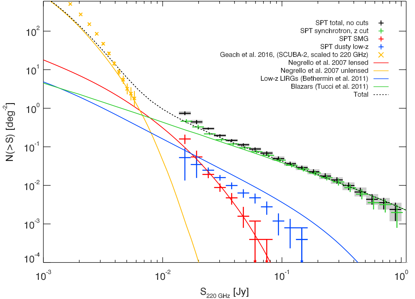
Figure 17. Cumulative number counts at 220 GHz for total, synchrotron-dominated, and dust-dominated source populations in the SPT-SZ catalog.
