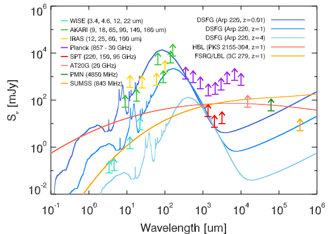
Figure 6. A comparison of survey depths for SPT and wide-field surveys used to cross-match with the SPT source catalog. Blue curves show example spectral energy distribution (SED) curves for dusty star-forming galaxies and their high-redshift component, SMGs, which are an Arp 220 SED shifted in redshift. Red and orange curves show two example synchrotron SEDs for different types of flat-spectrum sources.
