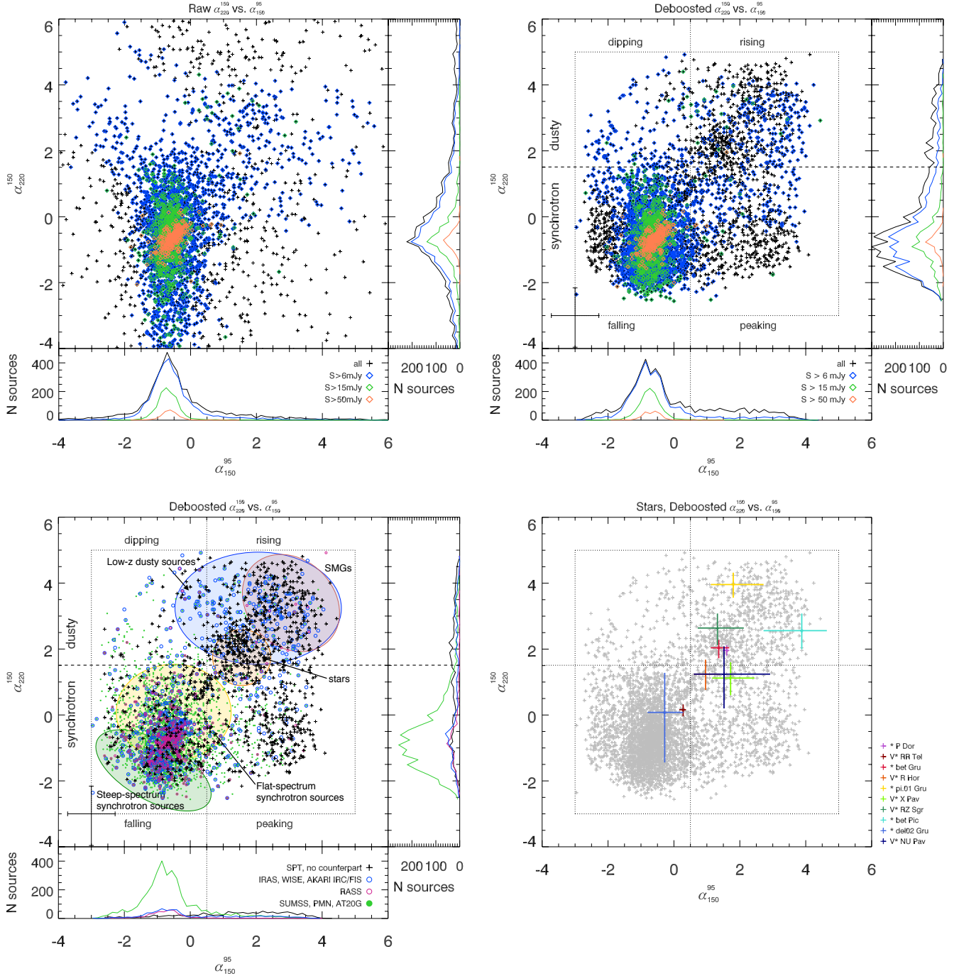
Figure 5. Upper panels: raw (left) and deboosted (right) \alpha_{150-220} vs. \alpha_{95-150} , where colors and symbols indicate flux level. Dotted box indicates the bounds of the prior on spectral index applied during deboosting, and dotted horizontal and vertical dashed lines indicate \alpha_{150-220} = 1.51 , the minimum of the 150-220 GHz summed posterior and the corresponding separation index between dusty and synchrotron in 95-150 GHz from reexamining the distributions of summed spectral index posteriors after population separation. These separation lines are used to categorize sources into four quadrants of “falling,” “rising,” “peaking,” and “dipping.” The typical error for a source at the 4.5- \sigma detection threshold is shown in the lower left corner of the deboosted spectral index plots. Lower panels: Left: deboosted \alpha_{150-220} vs. \alpha_{95-150} , where colors and symbols indicate cross-matches with external catalogs, and black crosses indicate SPT sources with no cross-matches in external catalogs. Right: Measured spectral indices for ten stars detected in the catalog, overplotted on the rest of the catalog, shown by grey crosses.
