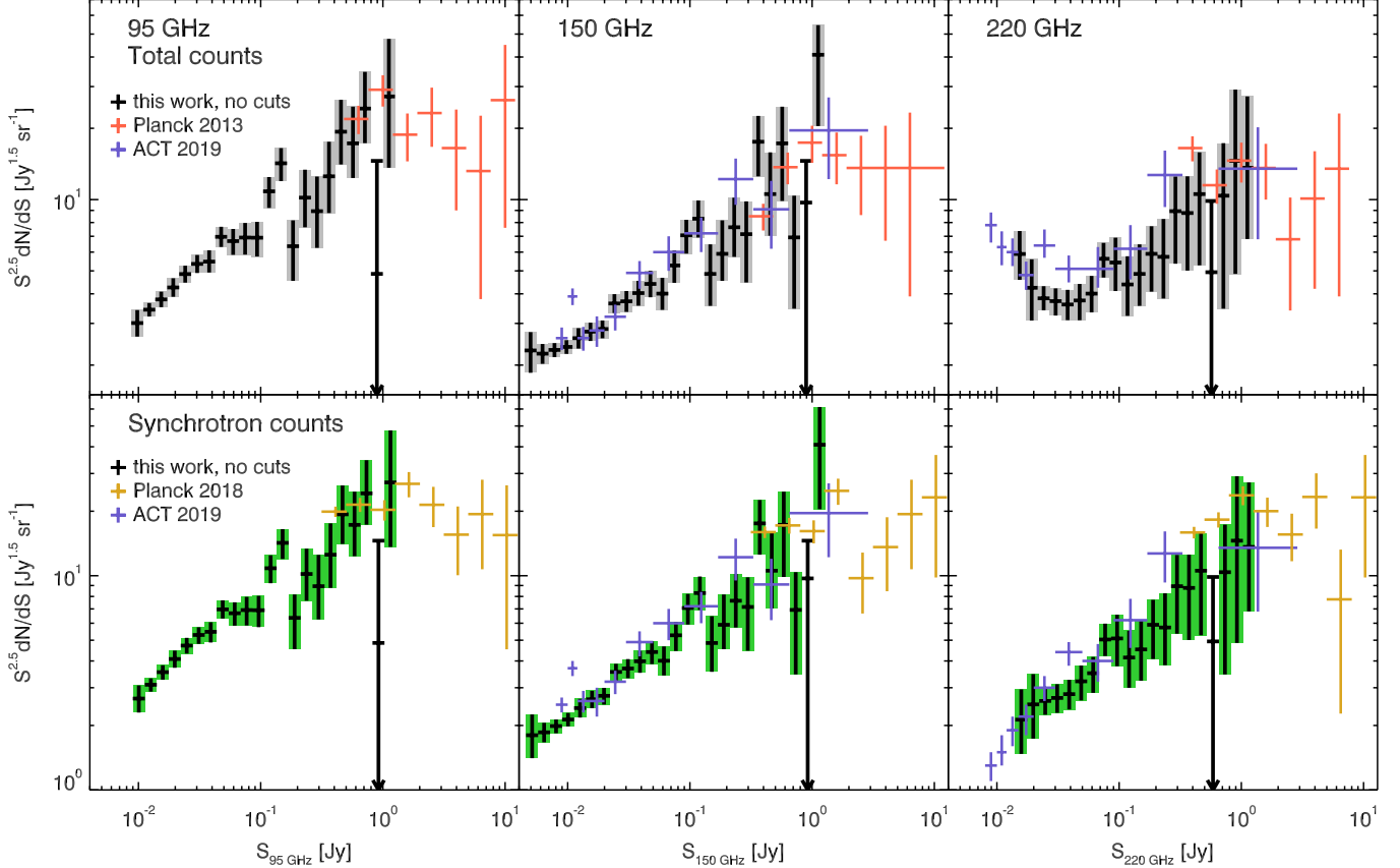
Figure 16. Upper: Total source counts (with no cuts applied other than removing sources identified as stars) for the current work, compared with total source counts from Planck (Planck Collaboration et al. 2013) and the Atacama Cosmology Telescope (ACT, Gralla et al. 2019). Lower: Synchrotron-dominated counts for the current work (shown with no cuts applied other than removing stars), compared with the Planck Multi-frequency Catalog of Non-thermal Sources (Planck Collaboration et al. 2018), where the counts were calculated applying the 70% Galactic mask, GAL070, and ACT AGN counts from Gralla et al. (2019).
