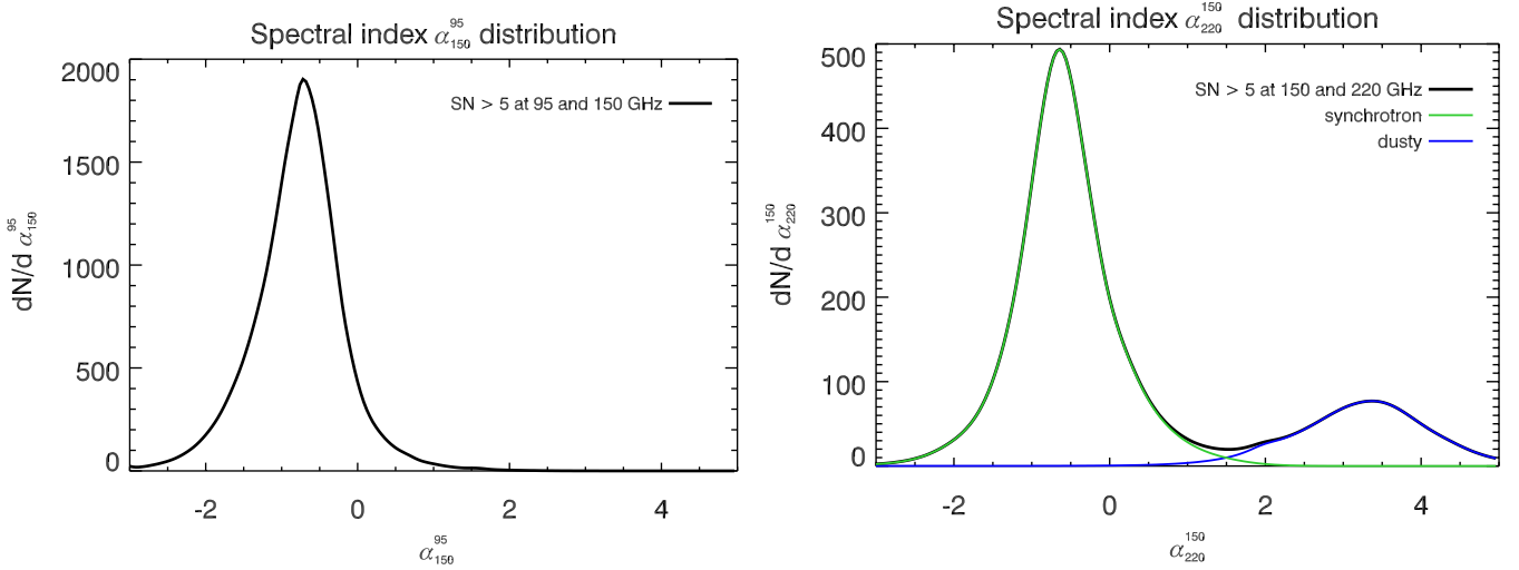
Figure 4. Summed normalized posterior distributions for the 95-150 GHz spectral index ( left ) and the 150-220 GHz spectral index ( right ), choosing for each spectral index only sources with detections above 5\sigma in both bands spanned by that index. As expected, the distribution for \alpha_{95-150}^{\max} shows a single peak at \alpha_{95-150}^{\max} \sim -0.7 \pm 0.6 , since synchrotron sources are expected to dominate at 95 GHz, especially for bright, and therefore high-signal-to-noise, sources. The distribution for \alpha_{150-220}^{\max} shows distinct peaks for synchrotron and dusty populations, with peaks at \alpha_{150-220}^{\max} \sim -0.6 \pm 0.6 and \alpha_{150-220}^{\max} \sim 3.4 \pm 0.8 , respectively, and we select the minimum at \alpha_{150-220}^{\max} = 1.51 as the threshold for applying a categorization for each source in the catalog.
