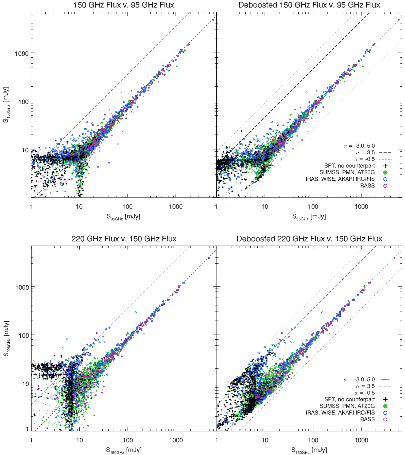
Figure 2. Upper panels: raw ( left ) and deboosted ( right ) fluxes for 150 GHz vs. 95 GHz for all sources in the catalog. Lower panels: raw ( left ) and deboosted ( right ) fluxes for 220 GHz vs. 150 GHz. Colors and symbols show cross-matches with external catalogs and black crosses indicate sources detected by the SPT-SZ survey with no counterparts in external catalogs. Dashed lines show expected spectral indices for synchrotron and dusty populations, and dotted lines in the right panels show bounds applied as priors on spectral index for the deboosting. The vertical and horizontal clusters of sources at relatively low flux in the left panels show the detection thresholds of 4.5\sigma , which translate to a different flux threshold for each field. For example, the clusters at clearly different flux levels in 220 GHz represent the 4.5\sigma thresholds in the double-depth fields and in the rest of the catalog.
