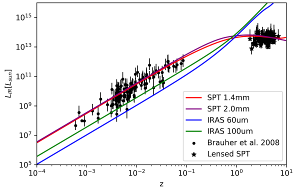
Figure 9. Observed infrared luminosity versus redshift for low-redshift infrared galaxies (Brauher et al. 2008) and SPT SMGs with detection thresholds for an Arp-220-like dusty galaxy spectrum shown in solid lines.
