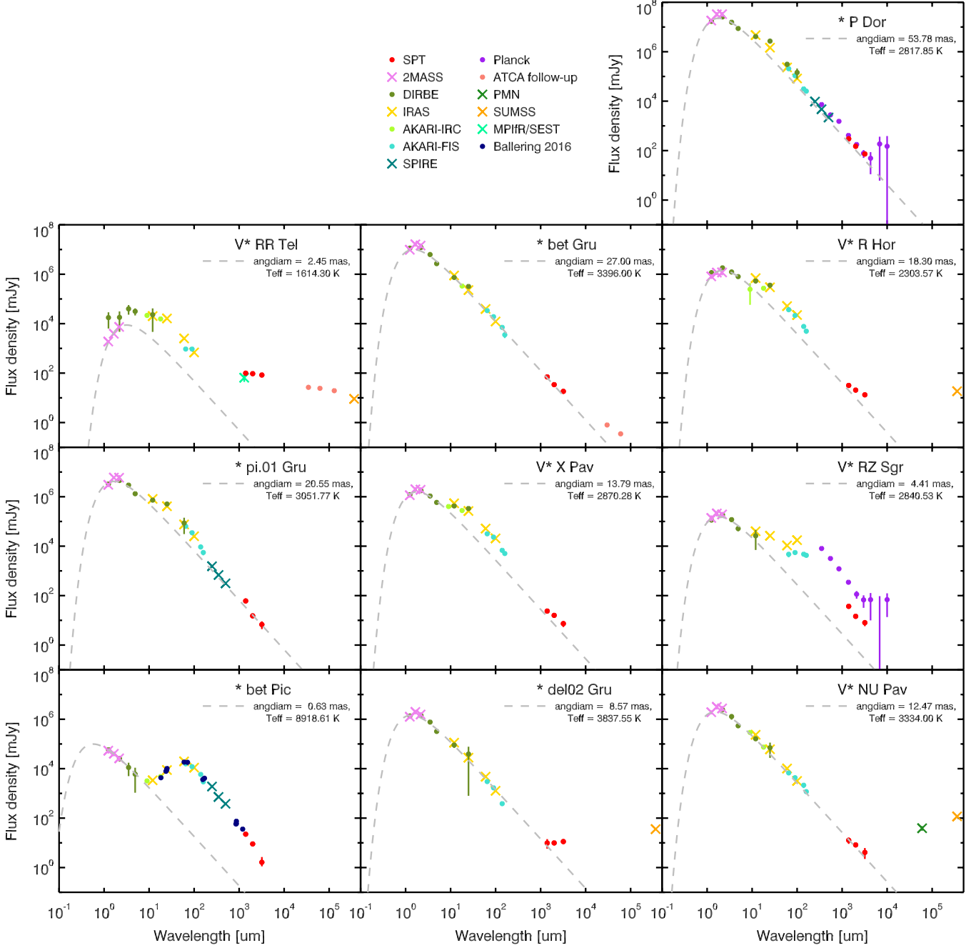
Figure 12. Spectral energy distributions for the ten stars detected in the SPT-SZ catalog, with flux measurements drawn from the literature. Grey dashed lines show blackbody model fits, where only fluxes from wavelengths in the range 1.25 - 5 \mu\text{m} are used in the fit. In addition to available statistical errors from the literature, 10% absolute calibration uncertainties have been applied to all fluxes from the literature.
