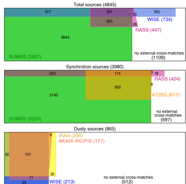
Figure 7. Venn diagrams showing fractional cross-match overlap between the SPT-SZ catalog and external catalogs. The top panel shows cross-matches with the full SPT-SZ catalog; the middle and bottom panels show cross-matches for synchrotron and dusty sources, respectively. In each panel, colored regions indicate the proportion of SPT-SZ sources with cross-matches in each catalog, showing overlapping cross-matches between various catalogs, and white space indicates the fraction of SPT-SZ sources that have no cross-matches with catalogs displayed in that panel. We find that of the 4845 total sources in the catalog, 1109 (23%) have no cross-matches in external catalogs; 597 of these are classified as synchrotron (15% of synchrotron sources), and 512 are classified as dusty (59% of dusty sources).
