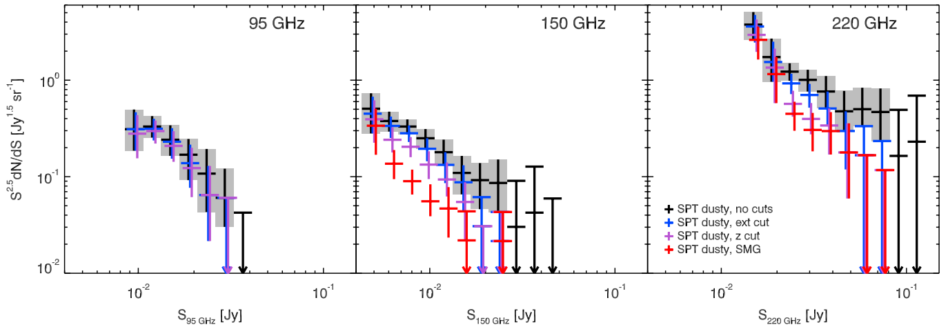
Figure 19. Number counts of SPT dust-dominated sources, showing a comparison of different cut versions. All sources identified as stars have been removed from the catalog prior to the counts calculation. Four cut versions are shown: 1) only stars have been removed, “no cuts.” 2) Cutting all stars and all sources flagged as extended or detected as multiple detections and confirmed to be from a single object, “ext cut,” 3) cutting all sources with measured redshifts z < 0.1 , “z cut,” and 4) the SPT SMG list, cutting all sources with measured redshifts, IRAS cross-matches, or dipping spectral behavior in the SPT bands.
