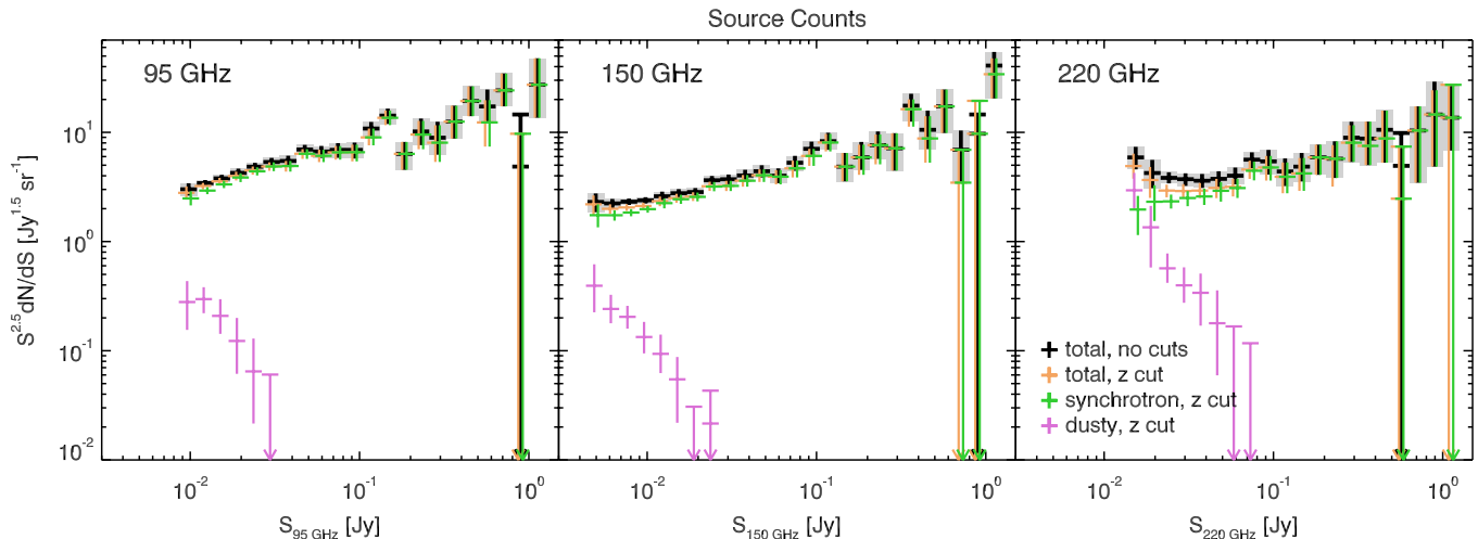
Figure 10. Differential number counts of emissive sources in 2530 square degrees of the SPT-SZ survey. Ten sources identified as stars have been removed. Two versions of the total counts are shown: total counts with no cuts applied, other than stars, and total counts with the “z cut” applied (cutting all objects with measured redshifts below z = 0.1 ). Counts for synchrotron-dominated sources (with “z cut” applied) are shown in green, and counts for dust-dominated sources (also with “z cut” applied) are shown in purple. Details of the cuts can be found in Section 4.10 and plots comparing cut versions for dusty and synchrotron counts can be found in the appendix.
