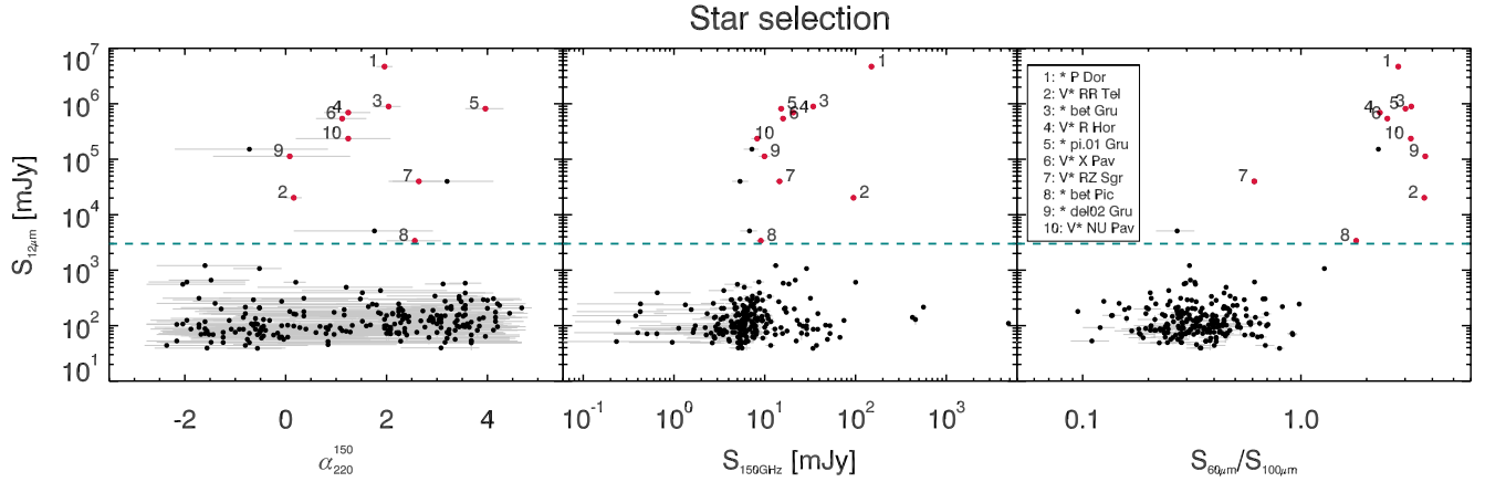
Figure 8. Cross-matched IRAS 12\ \mu\text{m} flux versus SPT spectral index \alpha_{150-220} ( left ), SPT flux at 150 GHz ( middle ), and the ratio of cross-matched IRAS 60\ \mu\text{m} flux to 100\ \mu\text{m} flux ( right ). Objects in the SPT-SZ catalog identified as stars are shown as red points, all other objects in the SPT-SZ catalog are shown as black points, with a rough separation threshold in 12\ \mu\text{m} flux shown as a teal dashed line. We note that using SPT data alone, stars are not distinguishable from non-stellar SPT sources (left two panels), and that while the ratio of 60\ \mu\text{m} to 100\ \mu\text{m} IRAS flux can be used to identify stars (right panel), high flux at 12\ \mu\text{m} is sufficient for star identification. The method for identifying stars is discussed in more detail in Section 4.9, and further details regarding stars identified in the SPT-SZ catalog and other sources that appear with high flux at 12\ \mu\text{m} but are not identified as stars can be found in Section 6.1.4.
