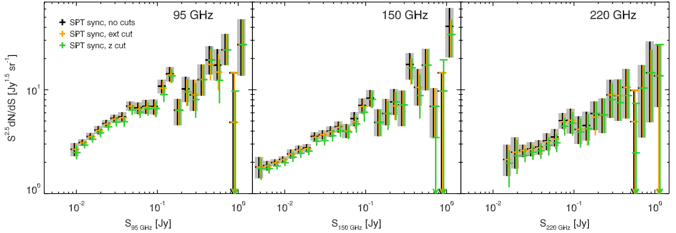
Figure 18. Number counts of SPT synchrotron-dominated sources, showing a comparison of different cut versions. All sources in the catalog that are identified as stars have been removed from the catalog prior to the counts calculation. Three cut versions are shown: 1) only stars have been removed, “no cuts.” 2) Cutting all stars and all sources flagged as extended or detected as multiple detections and confirmed to be from a single object, “ext cut,” and 3) cutting all sources with measured redshifts z < 0.1 , “z cut.”
