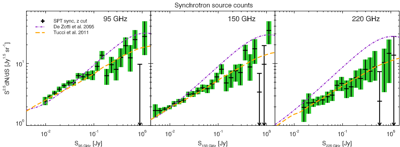
Figure 13. Differential number counts of SPT synchrotron-dominated sources. All sources in the catalog that are identified as stars as well as all sources flagged with the “z cut” (i.e. sources with measured redshifts z < 0.1 ) have been removed from the catalog prior to the counts calculation. A comparison of the effects of different cut versions on the number counts can be found in the appendix. Overplotted are the De Zotti et al. (2005) and the Tucci et al. (2011) models, which have not been fit to the SPT data.
