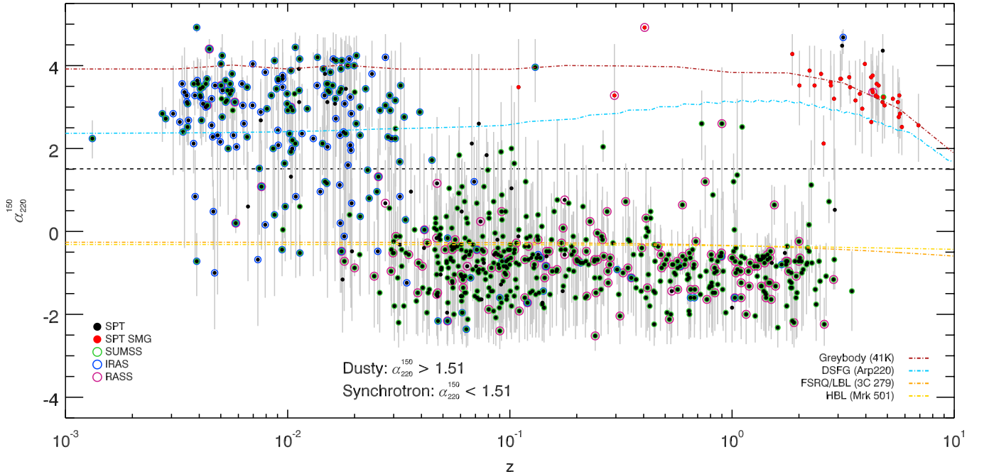
Figure 11. Deboosted \alpha_{150-220} versus redshift for sources in the SPT-SZ catalog with measured redshifts either from cross-matches in NED or follow-up observations with ALMA (Weiß et al. 2013; Strandet et al. 2016). Sources in the SMG list with measured redshifts are shown as red points, all other SPT-SZ catalog sources are shown as black points. The black dashed line shows the separation between dusty and synchrotron sources. Dot-dashed lines show two models of dusty sources: a 41 K greybody (red) and an Arp 220 model (blue), and two models of flat-spectrum synchrotron sources: a model for flat-spectrum sources dominated by radio emission (FSRQs and LBLs) based on the spectrum of the blazar 3C 279, and a model for flat-spectrum sources dominated by X-ray emission (HBLs) based on the spectrum of the blazar Markarian 501. Because redshifts are drawn from multiple sources, the selection function for SPT-SZ sources with measured redshifts is complicated. We don’t attempt to quantify the redshift completeness of the catalog, and this figure therefore is meant to illustrate the known redshift information for the catalog.
