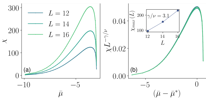
FIG. 4. (a) Susceptibility for structure C and \bar{T} = 1.5 for volumes of length L = 12 ( N=217 ), L = 14 ( N=126 ) and L = 16 ( N=125 ). (b) Collapse of the susceptibility curves (inset: a power law fit to estimate \gamma ).
