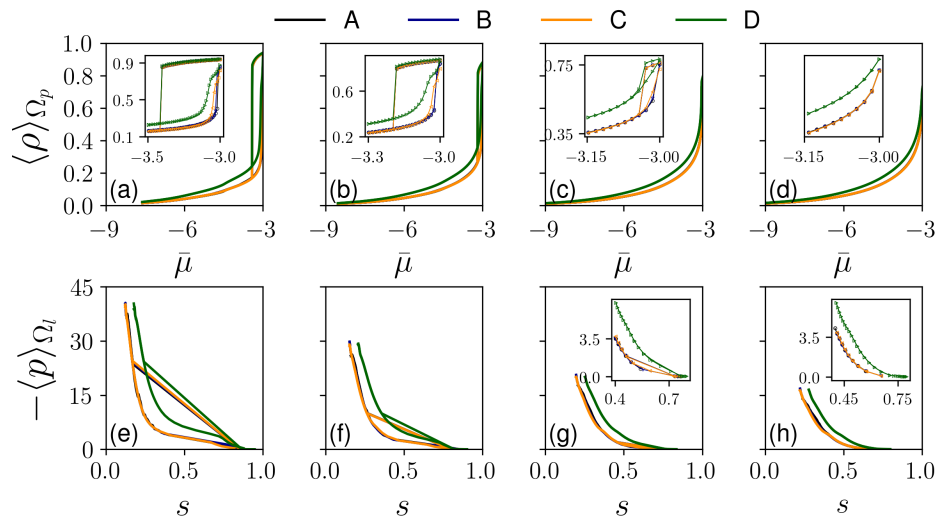
FIG. 2. Isotherms (a)-(d) and capillary pressure curves (e)-(h) for granular packings at \bar{T} = 1.0 , \bar{T} = 1.2 , \bar{T} = 1.4 and \bar{T} = 1.5 , respectively.
