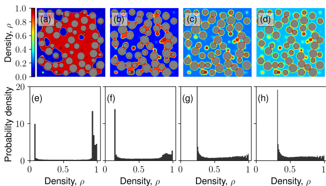
FIG. 3. (a)-(d): Spatial distribution of density fields, \rho(\vec{x}) , for granular packing C and at cross-sections corresponding to z = 44 nm, h = 0.96 and (e)-(h): Probability density for the density fields (coarse-grained over L^3 = 1 nm 3 ) for the same structure at h = 0.96 for \bar{T} = 1.0 , \bar{T} = 1.2 , \bar{T} = 1.4 and \bar{T} = 1.5 , respectively.
