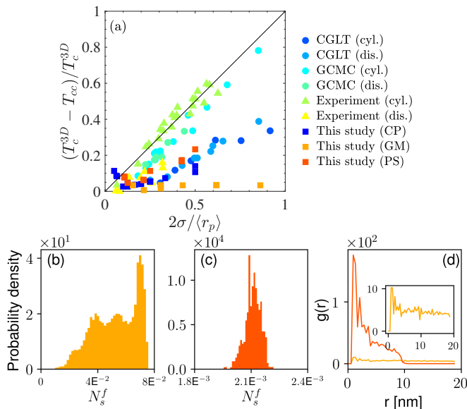
FIG. 1. (a) Shift in capillary critical temperature T_{cc} as a function of the ratio 2\sigma/\langle r_p \rangle . Previous simulations (circle) and experimental (triangle) data from literature [33] along with our results (square) for all the considered cylindrical pores (CP), porous solids (PS) and granular media (GM) and for various space discretizations a_0 , where a_0 \sim \sigma . (b) and (c) N_s^f ( r = 20 nm) of GM and PS, respectively, for structure C . (d) Partial radial distribution function for a fluid site at the pore-solid interface with a connected path to a solid site at the pore-solid interface.
