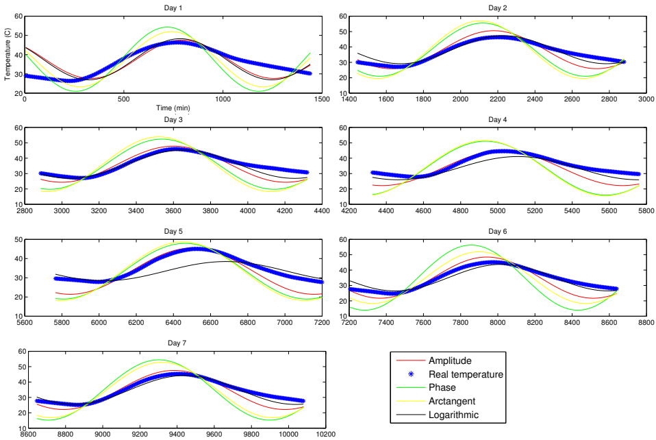
Figure 3. Temperature distributions.
