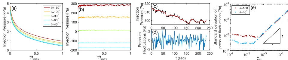
FIGURE 3. (a)-(b) Temporal evolution of the injection pressure at Ca = 10^{-3} and Ca = 10^{-7} respectively. At high Ca , the injection pressure decreases as the viscous fingers approach the outer boundary of the flow cell. At low Ca , the injection pressure is dominated by Laplace pressure fluctuations at the interface. We use wavelet decomposition (Cai 2002; Sygouni et al. 2006, 2007) to split the pressure signal ( Ca = 10^{-5} and \theta = 160^\circ here) into its (c) global trend and (d) cyclic component. (e) The standard deviation of the pressure fluctuations point at two different regimes. At low Ca , pressure fluctuations are dominated by stick-slip changes in Laplace pressure. At high Ca , pressure fluctuations are dominated by changes in the effective hydraulic conductance of dominant flow channels.
