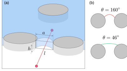
FIGURE 4. (a) Pore-scale perspective for the scaling of pressure fluctuations. The diagram shows a typical pore being invaded. The characteristic distance between the pore centers is l (red line), the pore height is h , and a characteristic throat size is a . (b) Typical configurations of the fluid-fluid interface in drainage and imbibition. Burst events are prevalent in drainage and the typical radius of out-of-plane curvature is of order a . Overlap events are prevalent in imbibition and the typical radius of out-of-plane curvature is an order of magnitude greater than a .
