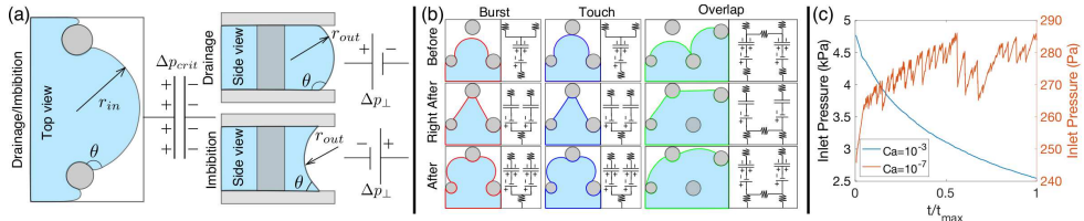
FIGURE 1. (a) Schematic diagram of in-plane and out-of-plane curvatures within the flow cell. Out-of-plane curvature represents the overall affinity of the porous medium to the invading fluid. It is determined by \theta and is analogous to a battery. In-plane curvature changes as the local interface evolves while pinned to a pore throat, and it is analogous to a capacitor. (b) Evolution of burst, touch, and overlap events. (c) Temporal profiles of the injection pressure bear close resemblance to similar experiments in the drainage regime at low (orange) and high (blue) Ca (Furuberg et al. 1996; Zhao et al. 2016).
