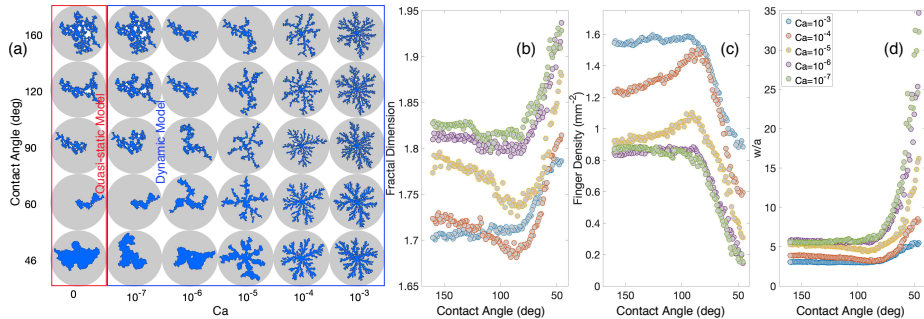
FIGURE 2. (a) Phase diagram of the invading fluid morphology at breakthrough; (b) Fractal dimension, computed by means of the box-counting method; (c) Number of fingers per unit area of injected fluid, which exhibits a maximum near \theta = 90^\circ ; (d) Normalized finger width ( w/a ) at different Ca and wettabilities measured at breakthrough. Finger width increases as the posts become more wetting to the invading fluid.
