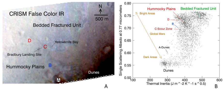
Figure 6. (a) Portion of CRISM false color image (also shown in Figure 5a) contrast enhanced to show local color variations. The surface becomes increasingly bright from the dunes toward the northwest. Data for locations A–D are discussed in the text and shown in Figures 6b and 7. (b) Scatterplot of single scattering albedo (SSA) derived from CRISM data versus thermal inertia from THEMIS, with key locations shown. Data retrieved for CRISM scene and same areas for THEMIS data. Global averages for dark and bright areas are also shown based on data provided in Putzig et al. [2005]. Note how data for areas covered by the CRISM scene show increasing thermal inertia with increasing SSA values, opposite to the main trend on Mars. Averages for the hummocky plains and bedded fractured units are shown, along with dunes to the south, and an average of 9 pixels (18 m/pixel) for the dark scour zone centered on the landing site.
