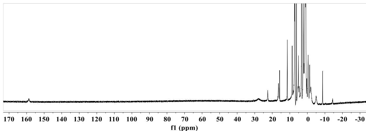
Figure S4.4. Wide view of the product mixture observed by ^1\text{H} NMR from the reaction between \text{P}_3^{\text{B}}\text{Co}(\text{H}_2) [\text{Co}](\text{H}_2)^\bullet and TEMPO ^\bullet .
