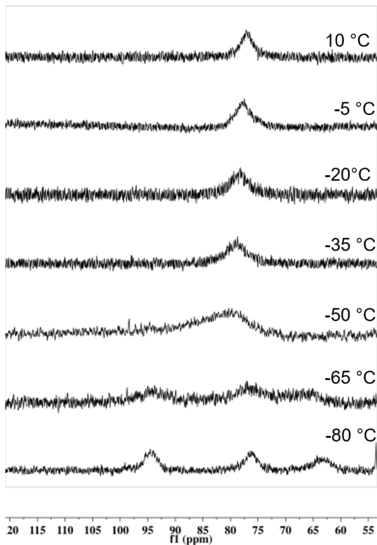
Figure S3.14. Variable temperature ^{31}\text{P} NMR (202 MHz) spectra highlighting the hydridic resonance(s) of [\text{Co}](\text{H})/[\text{Co}](\text{H})(\text{H}_2) in toluene- d_8 under an \text{H}_2 atmosphere from 10 °C (top) to -80 °C (bottom).
