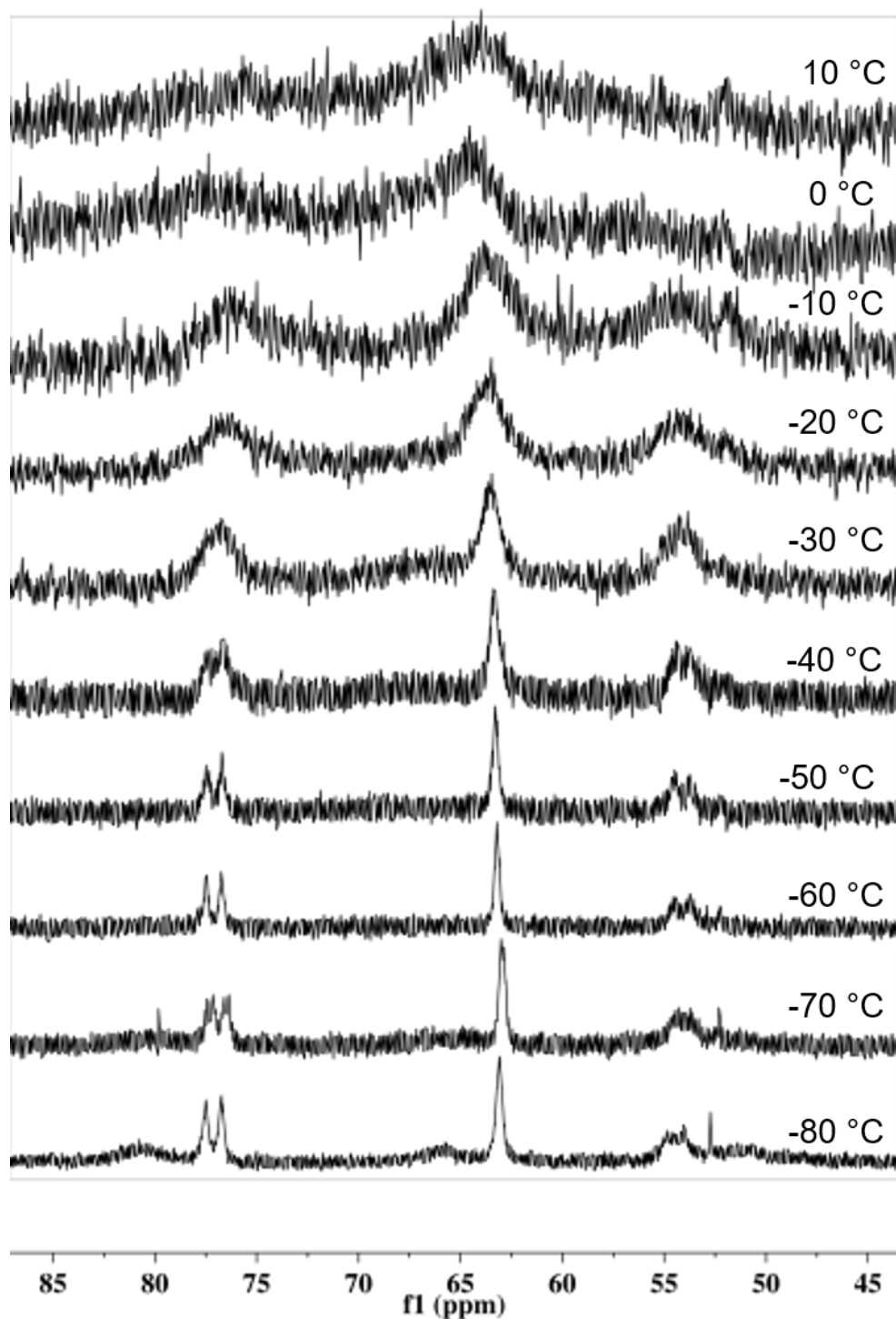
Figure S3.17. Variable temperature ^{31}\text{P} NMR spectra (202 MHz) of [\text{Co}](\text{H})/[\text{Co}](\text{H})(\text{N}_2) in \text{toluene-}d_8 under an \text{N}_2 atmosphere from 10\text{ }^\circ\text{C} (top) to -80\text{ }^\circ\text{C} (bottom).
