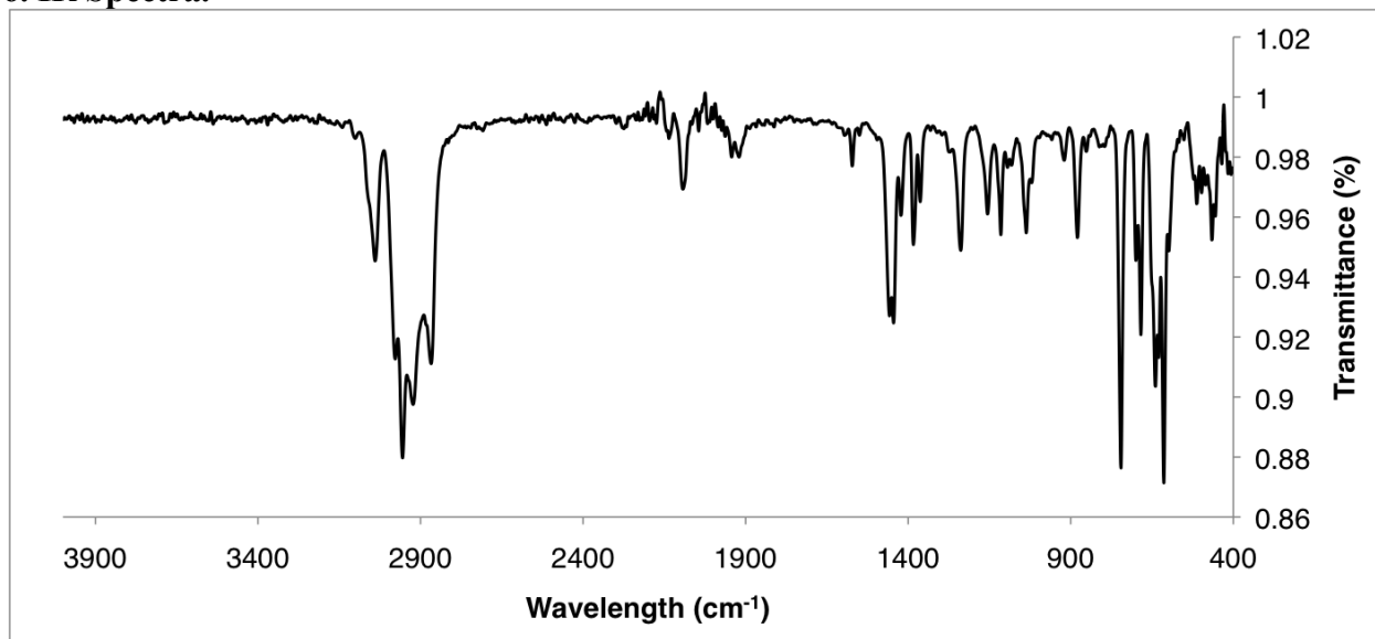
Figure S6.1. IR spectrum of P_3^B\text{Co}(\text{H}) [\text{Co}](\text{H})/[\text{Co}](\text{H})(\text{N}_2) collected as a thin film under an \text{N}_2 atmosphere ( \nu_{\text{Co-H}} = 1943 \text{ cm}^{-1} ). The weak sharp stretch at 2092 \text{ cm}^{-1} is reproducibly observed and may be attributable to the equilibrium \text{N}_2 ligation observed by alternative spectroscopies (UV-Vis, NMR). Alternatively, this may be due to the presence of a minor P_3^B\text{Co}(\text{N}_2) impurity, with a reported \text{N}_2 stretch at 2089 \text{ cm}^{-1} within the error of the instrument.
