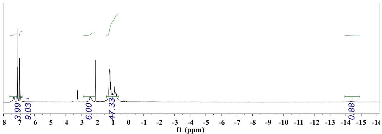
Figure S3.7. ^1\text{H} NMR spectrum (500 MHz) of [\text{Co}](\text{H}) in toluene- d_8 under vacuum.
