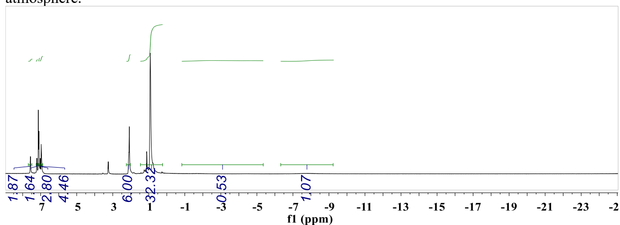
Figure S3.6. ^1\text{H} NMR spectrum (500 MHz) of [\text{Co}](\text{H})/[\text{Co}](\text{H})(\text{H}_2) in \text{toluene-}d_8 under an \text{H}_2 atmosphere at 10\text{ }^\circ\text{C} .
