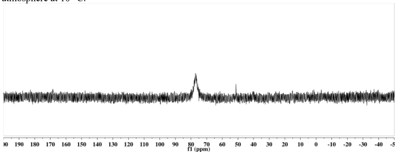
Figure S3.9. ^{31}\text{P} NMR spectrum (202 MHz) of [\text{Co}](\text{H})/[\text{Co}](\text{H})(\text{H}_2) in toluene- d_8 under an \text{H}_2 atmosphere.
