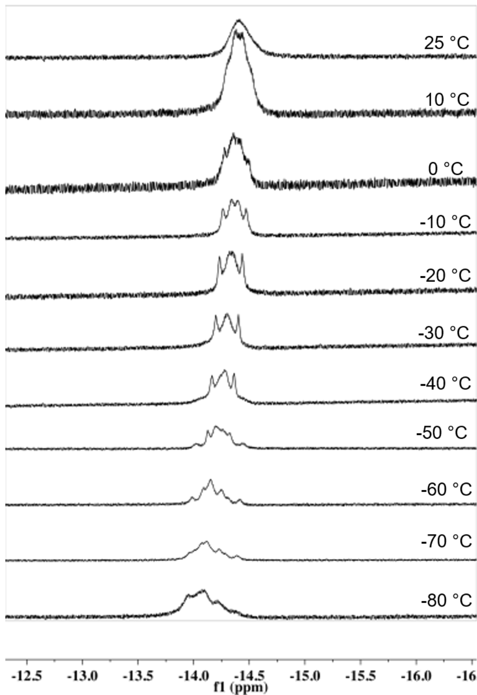
Figure S3.18. Variable temperature 1 H NMR (500 MHz) spectra highlighting the hydridic resonance of [Co](H)/[Co](H)(N 2 ) in toluene- d 8 under an N 2 atmosphere from -80 °C (bottom) to 25 °C (top).
