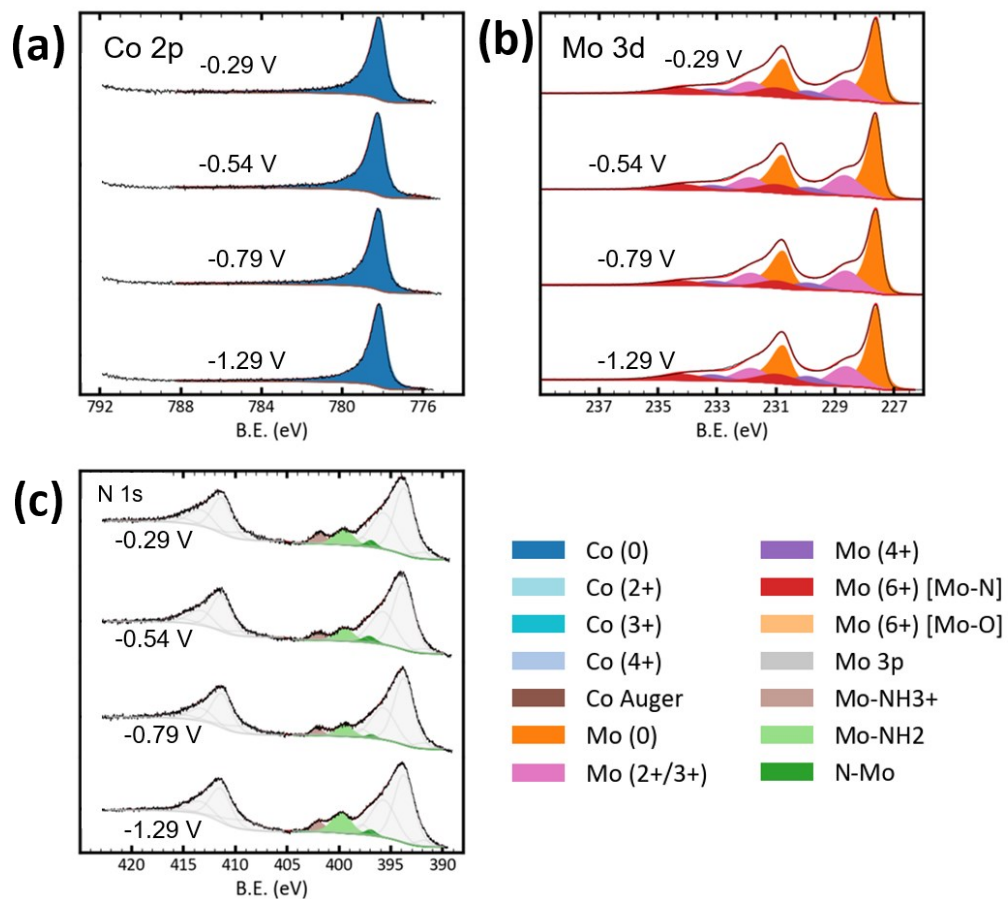
Figure S9. X-ray photoelectron spectra of the n^+ -Si/Ti/CoMo surface after 20 min of electrocatalysis in aqueous 50 mM H_2SO_4 electrolyte at four different potentials vs. RHE. (a) Co 2p core levels; (b) Mo 3d core levels and (c) N 1s core levels. Color coding is given in the legend; B.E. is the binding energy.
