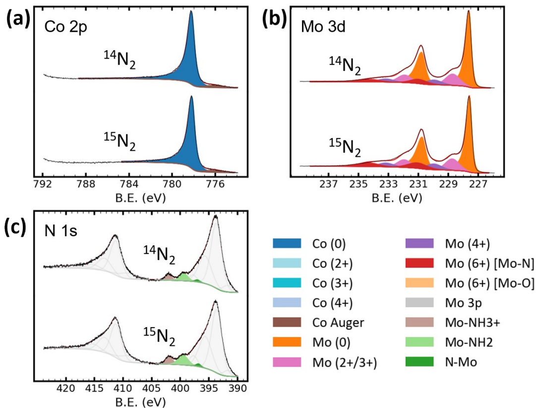
Figure S8. X-ray photoelectron spectra of the n^+ -Si/Ti/CoMo surface after 20 min of electrocatalysis in aqueous 50 mM H_2SO_4 electrolyte at -0.54 V vs. RHE under ^{14}N_2 purging (top) and ^{15}N_2 purging (bottom). (a) Co 2p core levels; (b) Mo 3d core levels and (c) N 1s core levels. Color coding is given in the legend; B.E. is the binding energy.
