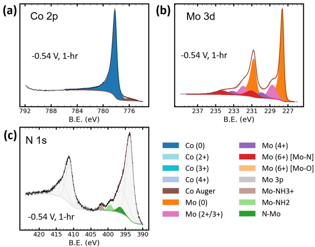
Figure S4. X-ray photoelectron spectra of the n^+ -Si/Ti/CoMo surface after 1 h of electrocatalysis in aqueous 50 mM H_2SO_4 electrolyte at -0.54V vs RHE. (a) Co 2p core levels; (b) Mo 3d core levels and (c) N 1s core levels. Color coding is given in the legend; B.E is the binding energy.
