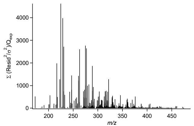
Figure S7 Diagnostic plots of PMF analysis on FIGAERO-CIMS measurements.
