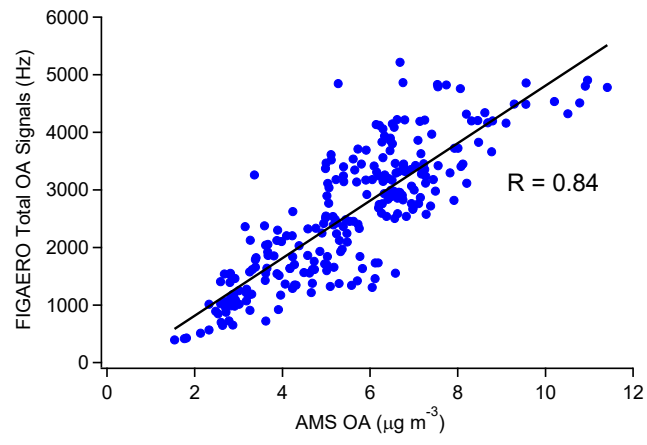
Figure S1 Correlation between FIGAERO total OA signals and AMS total OA mass concentration.
