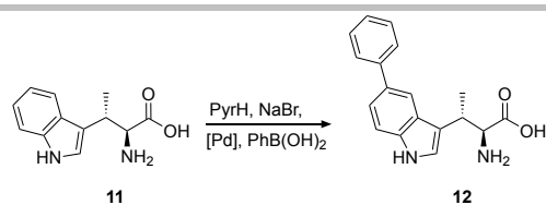
Scheme 4. One-pot C 5 -arylation of \beta -methylTrp ( 11 ). Flavin-dependent Trp-halogenase PyrH brominates C 5 , which then participates in a palladium-catalyzed Suzuki cross-coupling to install the aryl group ( 12 ). [66]
