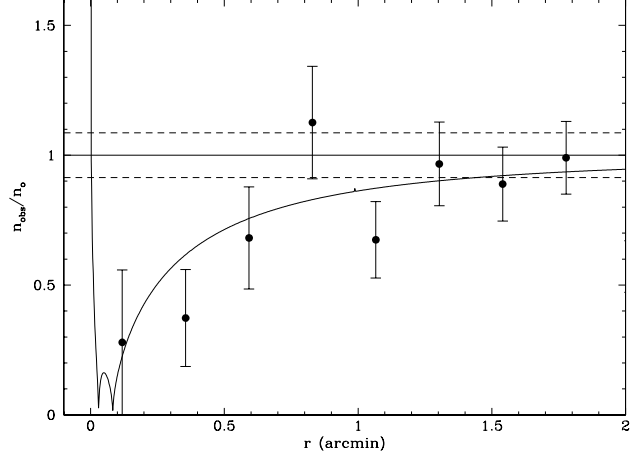
Figure 9. The radial depletion curve for a NFW cluster with r_s = 125h^{-1} kpc and c = 6 . The inner dip corresponds to the radial arc at x_r = 2 arcsec while the outer dip corresponds to the tangential arc at x_t = 5 arcsec, for a source population with \alpha = 0.185 . Overlaid are the points the Abell 2219 depletion curve, as in Fig. 7.
