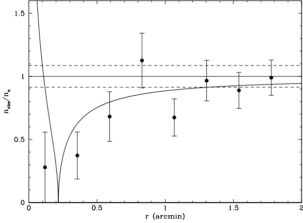
Figure 7. Ratio of observed number density to unlensed number density of red galaxies with distance from the cluster centre, using a bin width of 14 arcsec. All measurements take into account the area in each bin obscured by the cluster galaxies. A depletion of number counts is clearly seen at small radii. The dashed lines indicate the errors in the measured value of n_0 , the unlensed number density (the effect of this uncertainty is considered in Section §4.3). The thick line shows the expected depletion profile induced by a SIS with \sigma_v \sim 800 \text{ km s}^{-1} .
