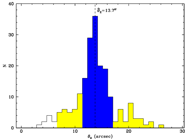
Figure 10. Distribution of the recovered \theta_E from 200 realizations of simulated lensing by an isothermal sphere, using the observed background population parameters ( n_0 = 20.3 \text{ arcmin}^{-2} , \alpha = 0.185 ). The darker shaded region indicates the resulting 66% confidence interval in the range 11.1 < \theta_E < 17.06 \text{ arcsec} , centred around the input value of \hat{\theta}_E = 13.7 \text{ arcsec} . The lighter shaded region indicates the 95% confidence interval in the range 6.8 < \theta_E < 26.5 \text{ arcsec} .
