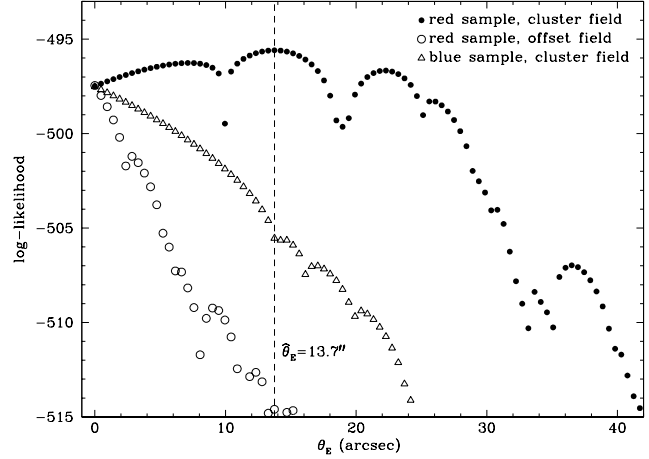
Figure 8. Maximum likelihood analysis for depletion of the red background galaxy sample (solid circles). The model corresponding to the peak is a SIS parametrized by the Einstein radius \hat{\theta}_E = 13.7 \text{ arcsec} . By contrast, the same analysis for the red galaxy sample in one of the offset fields (open circles) peaks at \theta_E = 0 \text{ arcsec} and shows no evidence of depletion, as does the sample of blue (foreground) galaxies in the cluster field (open triangles). The curves have been vertically shifted to the same zeropoint for clarity.
