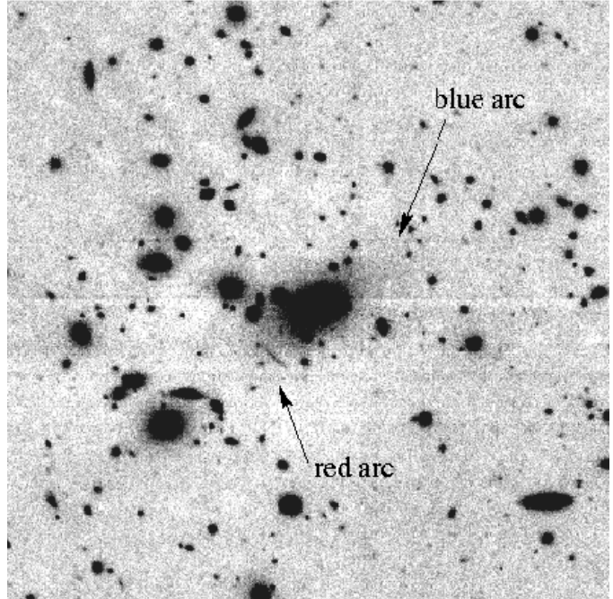
Figure 6. The central 2.7 \times 2.7 arcmin of the H -band CIRSI image, showing the red arc reported in Smail et al. (1995a). The second, bluer arc system is only barely visible in this infrared image.
