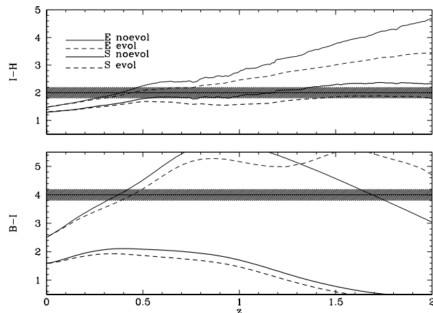
Figure 1. Dependence of optical-infrared and optical-optical colour on redshift for early- and late-type galaxies derived from the GISSSEL96 spectrophotometric codes (Bruzual & Charlot, in preparation) with and without evolution. The shaded area shows a range of colour when taking into account typical photometric errors of \pm 0.2 for the measurement of a typical early-type cluster sequence at intermediate redshift. Clearly the addition of the infrared magnitude reduces the dependence of colour on spectral type and allows for a more efficient selection of a background population. This is an obvious advantage over using optical colours alone to distinguish between foreground and background populations.
