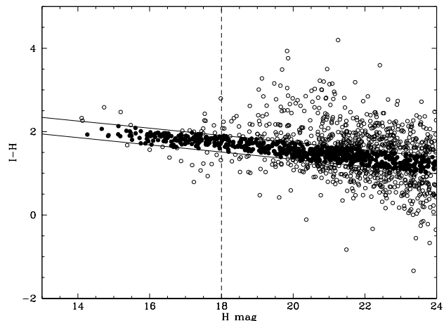
Figure 4. Colour-magnitude diagram for all objects in the cluster field. The cluster galaxies are indicated by filled circles; the population of objects selected for lensing purposes are those with colours redder than the cluster sequence and with 18 < H < 24 (dashed line).
