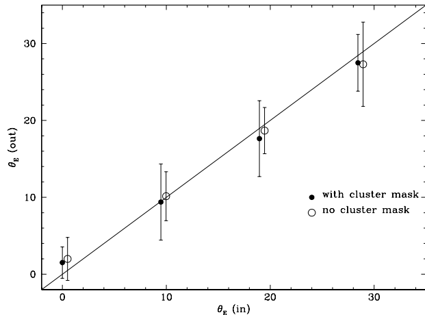
Figure 11. Simulations showing recovered \theta_E vs input \theta_E , with and without a cluster mask (the open circles are offset slightly in the +x direction for clarity). The cluster mask, which obscures about 10% of the field including much of the central region, has no significant effect on the recovered \theta_E (aside from increasing the errors), even given the low numbers of background galaxies.
