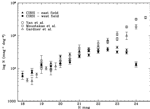
Figure 3. Comparison of the CIRS I H -band number counts with those from the literature. Shown are the two CIRS I offset fields (covering 27 \text{ arcmin}^2 each), the Yan et al. (1998) H -band survey, and the Gardner et al. (1993) and Moustakas et al. (1997) K -band surveys. For comparison purposes the K -band points have been shifted by one magnitude according to the approximation H - K = 1 . The counts from the literature have all been corrected for incompleteness at faint magnitudes.
