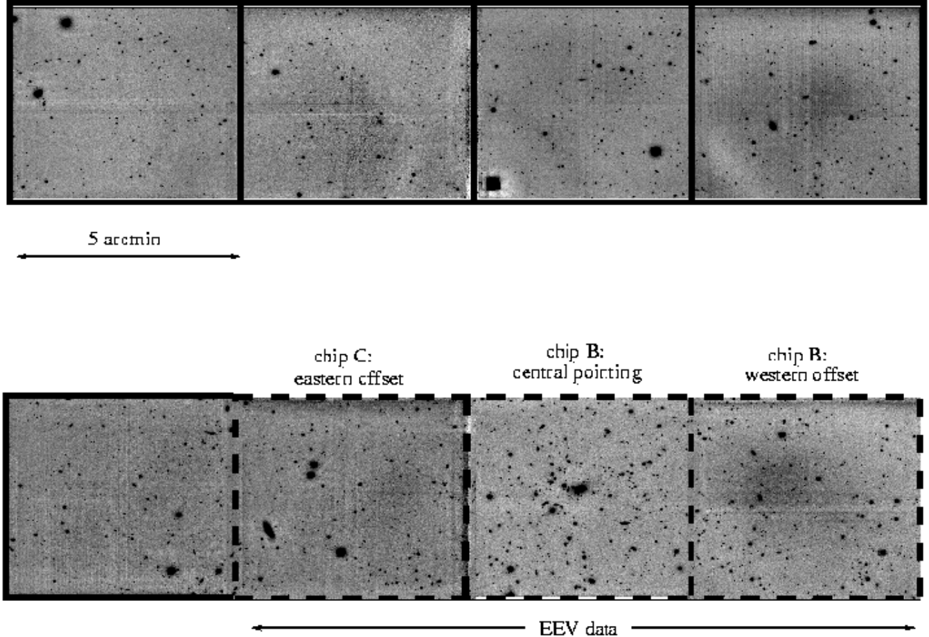
Figure 2. The field of view of CIRSI after two adjacent pointings. The resulting two strips each measure \sim 20 \times 5 arcmin. The dashed lines indicate the region which overlapped with the optical data. Treating the individual CIRSI chips as separate images, the western offset field, central cluster field, and eastern offset field (all with overlapping optical data) are labelled. North is up, east is to the left.
