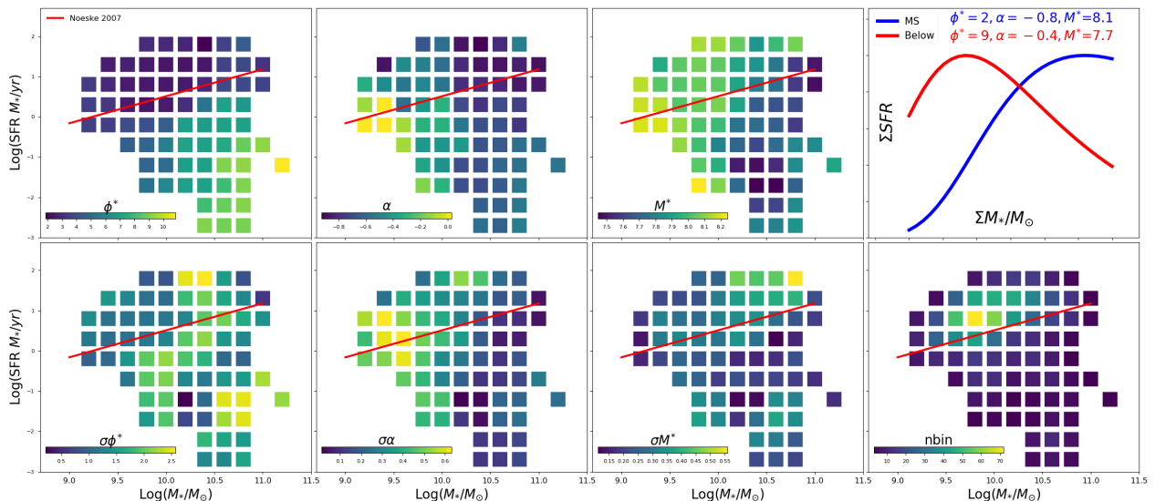
Figure 3. Schechter parameters best fitted to the resolved main sequence of individual galaxies are shown on the binned integrated stellar mass-SFR plane. Left-three columns show the median (top) and standard deviation (bottom) of \phi^* , \alpha , and M^* . Red solid line shows the main sequence of star-forming galaxies at z \sim 1 to guide the eye. Top-right panel shows two Schechter functions with average value of galaxies on and two dex below the main sequence at \text{Log}(M_*/M_\odot) \sim 10.5 . Bottom-right panel shows number of galaxies in each bin of SFR and stellar mass.
