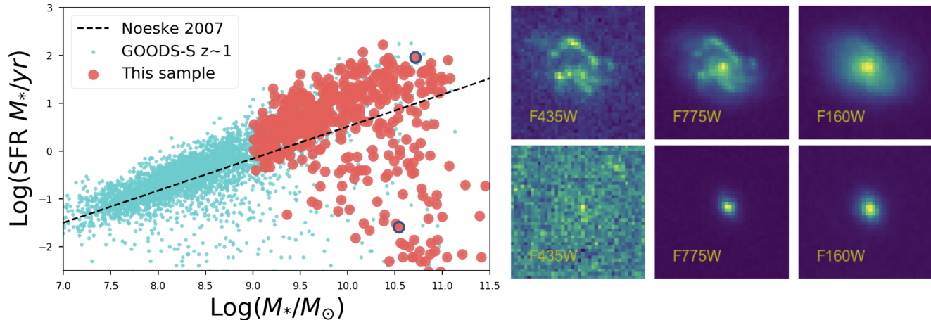
Figure 1. Left:Galaxies selected for this study are shown as red circles on top of all GOODS-S galaxies at z \sim 1 shown with cyan dots. Black dashed line shows the main sequence of star forming galaxies at this redshift from Noeske et al. (2007). Right: HST cutouts in F435W, F775W, and F160W of a star forming and quenched galaxy on top and bottom panels, respectively.
