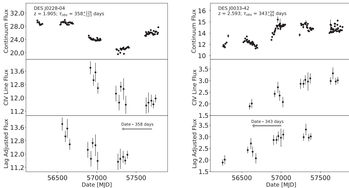
Figure 6. Light curves of the two OzDES AGNs in this study including the continuum flux represented by the DES g -band photometry ( top panel ) and CIV line flux measured from the OzDES spectra ( middle panel ). The CIV line light curve adjusted by the measured time lag is shown in the bottom panel . Fluxes are in units of 10^{-17} \text{ erg s}^{-1} \text{ cm}^{-2} \text{ \AA}^{-1} .
