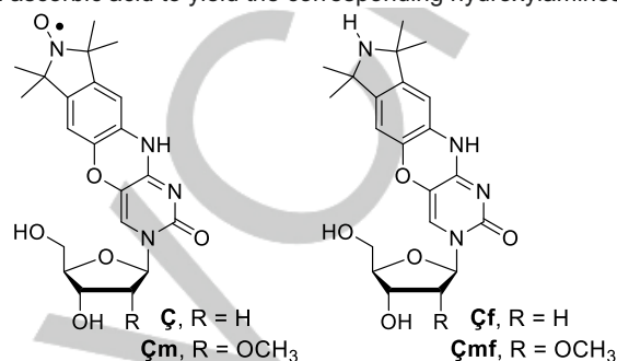
Figure 1. The rigid spin labels Ç [16] and Çm [26] and their corresponding amines Çf [16] and Çmf [27] .
