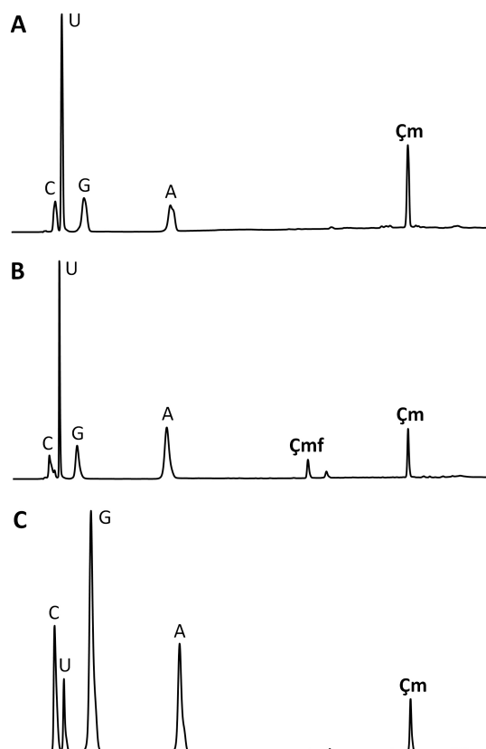
Figure 3. HPLC chromatograms of RNA oligonucleotides after enzymatic digestion with snake venom phosphodiesterase, nuclease P1 and alkaline phosphatase. A. Crude RNA I (5'-UGCAU \zeta\mathbf{m} UU-3') synthesized using 4 . B.
