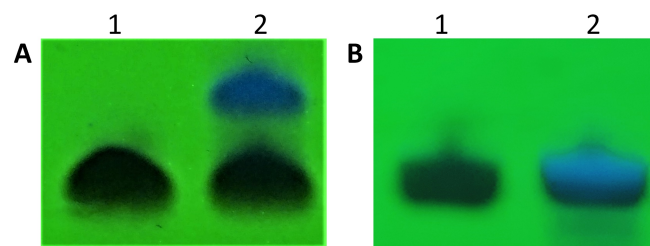
Figure 2. Analysis of spin-labeled oligonucleotides by DPAGE. A. Crude 8-mer RNA oligonucleotides I (lane 1) and II (lane 2) (5'-UGCAU \zeta\mathbf{m} UU-3'), synthesized using 4 and the phosphoramidite of unprotected \zeta\mathbf{m}^{[26]} respectively. B. Crude 21-mer DNA oligonucleotides IV (lane 1) and V (lane 2) (5'-d(PhO-TGAGGTAGTAGGTTGTATA \zeta\mathbf{T} )-3'), synthesized using 3 and the phosphoramidite of unprotected \zeta\mathbf{C}^{[16]} respectively. PhO is a phosphate.
