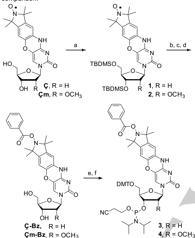
Figure 2. Analysis of spin-labeled oligonucleotides by DPAGE. A. Crude 8-mer RNA oligonucleotides I (lane 1) and II (lane 2) (5'-UGCAU \zeta\mathbf{m} UU-3'), synthesized using 4 and the phosphoramidite of unprotected \zeta\mathbf{m}^{[26]} respectively. B. Crude 21-mer DNA oligonucleotides IV (lane 1) and V (lane 2) (5'-d(PhO-TGAGGTAGTAGGTTGTATA \zeta\mathbf{T} )-3'), synthesized using 3 and the phosphoramidite of unprotected \zeta\mathbf{C}^{[16]} respectively. PhO is a phosphate.
