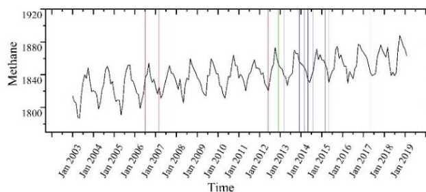
Fig. 3: Trend of Methane.
