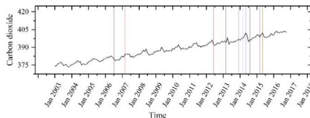
Fig. 2: Trend of Carbon dioxide.
