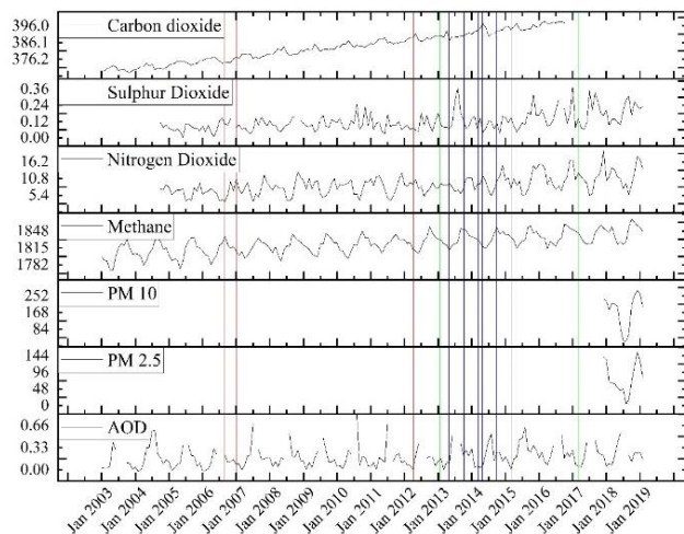
Fig 1: Trend of trace gases under observation. The straight lines in the figure mark the installation of new thermal power plant. The Red lines label for NTPC, Green for Essar, Blue for Reliance and Orange for Hindalco.
