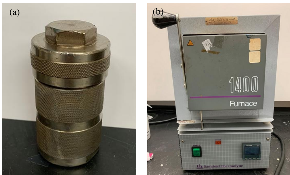
Figure 3.3 (a) Teflon lined stainless steel autoclave (b) A Barnstead Thermolyne furnace 1400.
