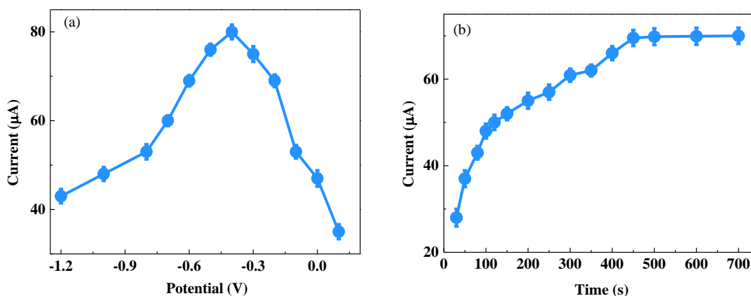
Figure 4.34 Optimization of the experimental conditions: Effects of (a) deposition potential (b) deposition time on the current responses of the 1T- WS_2 modified GCE for 1 mM Hg^{2+} . Data were presented as mean \pm s.d. (n = 3).
