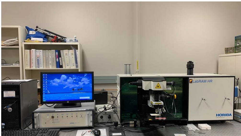
Figure 3.11 Experimental setup for a LABRAM HR Raman spectrometer.
