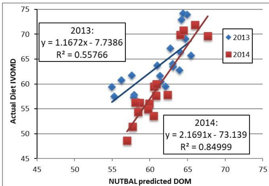
Figure 2. Regression of actual dietary in vitro organic matter digestibility (IVOMD) on fecal NIRS prediction of dietary digestible organic matter (DOM) to validate ability of fecal NIRS to predict actual dietary IVOMD. Regression relationships differed among years ( P < 0.05 ). Coefficient of variation ( r^2 ) estimates proportion of variation in actual values explained by predicted values. R^2 values range from 0 to 1 with those closer to 1 being better. The regression intercept should be 0 and slope should be 1 for a 1:1 relationship between predicted and actual values. Intercept and slope were similar to 0 and 1 ( P > 0.05 ), respectively, in 2013, but differed from 0 and 1 ( P < 0.05 ) in 2014.
