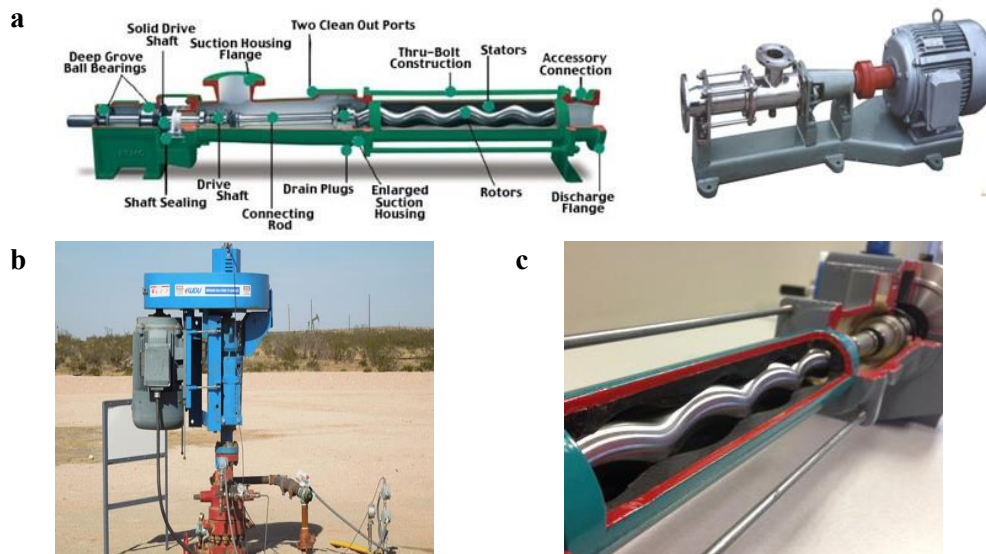
Figure 1. a) PCP system components b) PCP system head c) Progressive cavities internal structure
