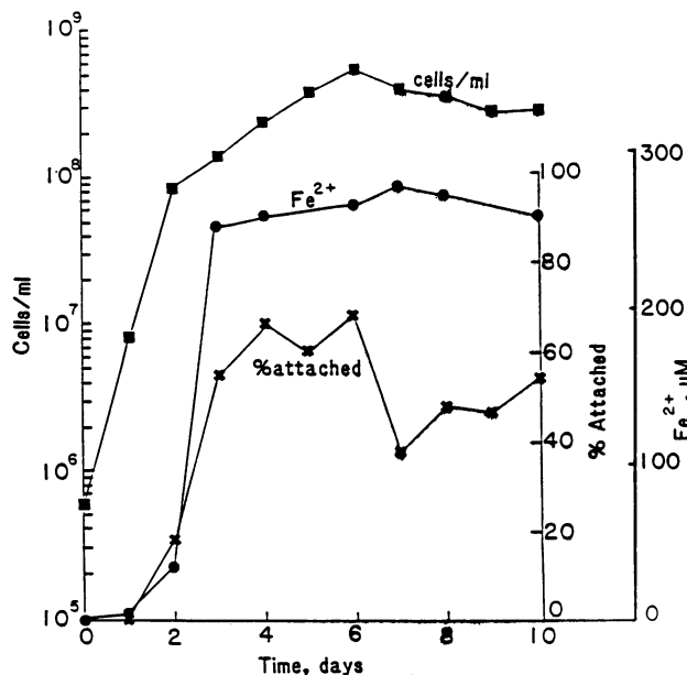
FIG. 5. Bacterial growth, percentage of cells attached to oxidized Fe particles, and Fe reduction in an enrichment culture.
