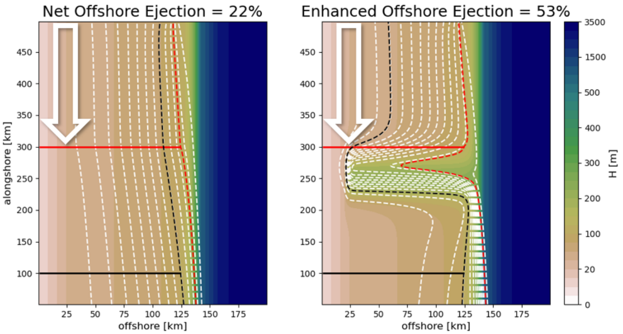
Figure 4: Resulting streamlines of two model runs are plotted as white dashed lines. On the left is of a run without a trough, and on the right is one with a baseline-parameter trough. White cartoon arrows are included to represent the shelf wind forcing, which is confined to only the shelf upwave of the trough location. Loss of shelf transport to the slope is quantified by calculating the difference in flow from the upwave (red) transect to the downwave (black) transect.
