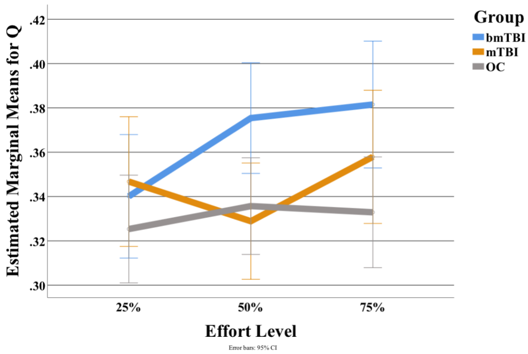
Figure 2. Modularity (Q) difference within groups and CE effort levels.
