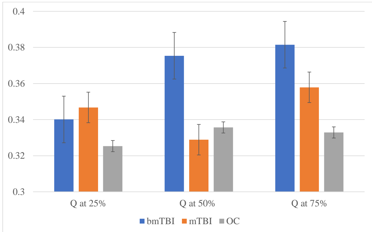
Figure 1. Modularity (Q) Difference between Groups and CE effort levels.
