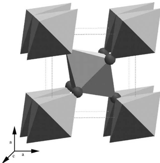
FIG. 6. The packing of \text{TiO}_6 octahedra in rutile.
