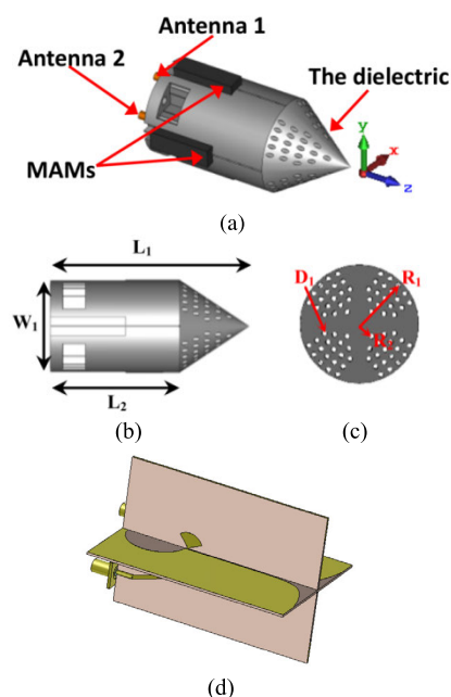
FIGURE 1. Geometry of the probe antenna: (a) the 3D view of the probe antenna; (b) the side view of the dielectric; (c) the front view of the dielectric; (d) the structure of Vivaldi antennas.
