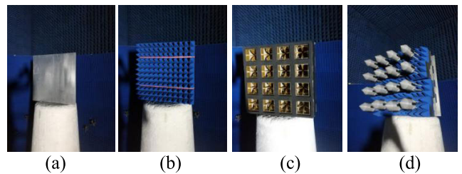
FIGURE 10. The different contrast models: (a) a flat metal plate; (b) a 12 × 12 pyramidal MAM array; (c) a 4 × 4 horn antenna array; (d) a 4 × 4 non-coplanar low-scattering probe antenna array.
