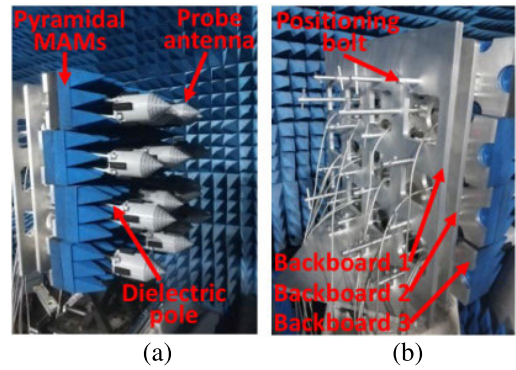
FIGURE 9. The prototype of the non-coplanar PWG: (a) the front view of the sub-array; (b) the back view of the sub-array.
