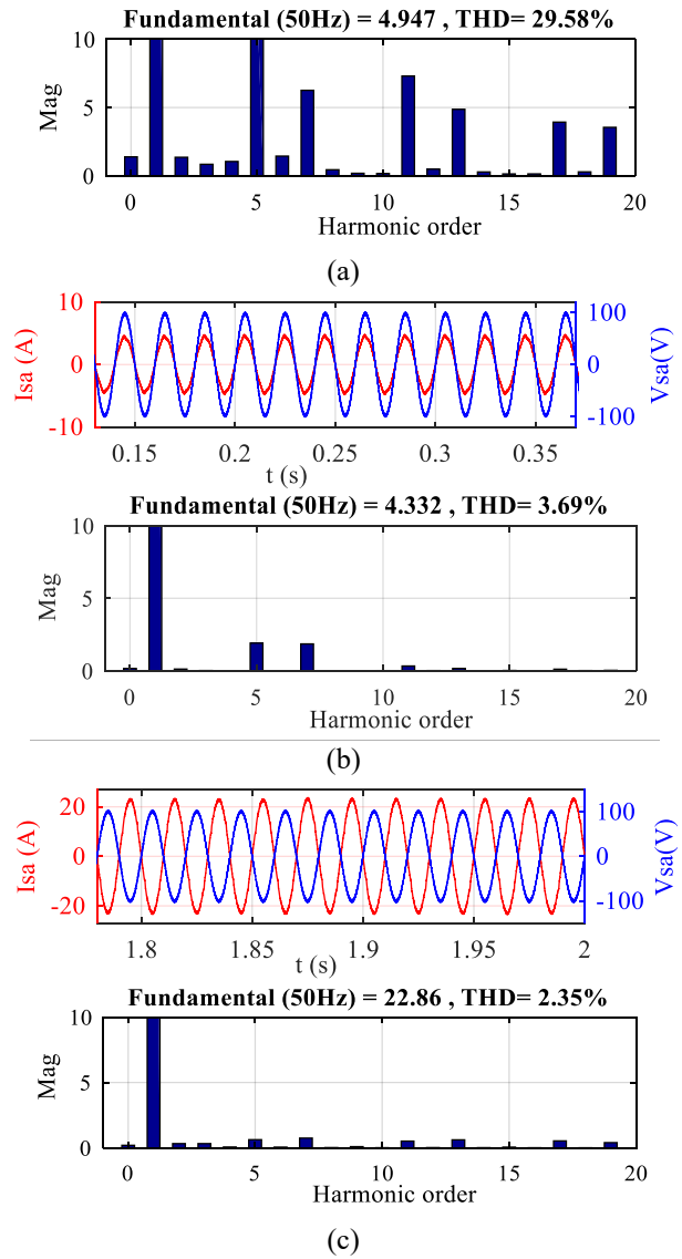
Figure 15. Source voltage and current with FFT of the latter of the SAPF based on conventional DPC equipped with the standard PID regulator: (a) without SAPF, (b) with SAPF and (c) with solar SAPF
