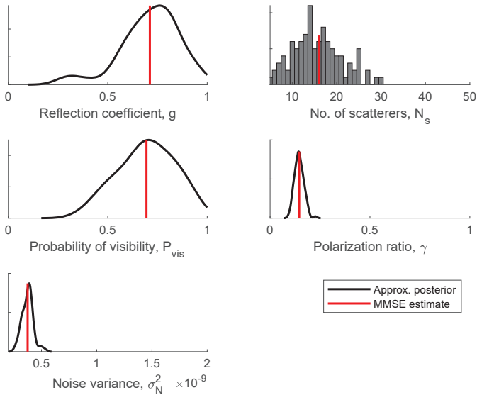
Fig. 5. Kernel density estimates of the approximate marginal posteriors for measured data after 10th iteration. The algorithm settings are same as given in Fig. 4.
