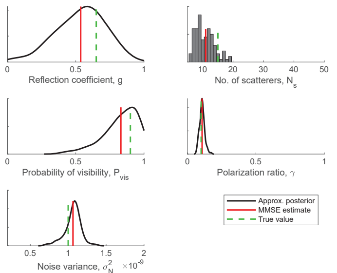
Fig. 4. Kernel density estimates of the approximate marginal posteriors for simulated data after N_{\text{iter}} = 10 iteration. Settings: L = 625 , J = 3 , M = 2000 , M_{\epsilon} = 100 , B = 4 GHz, K = 801 , \Delta f = 5 MHz, t_{\text{max}} = 200 ns.
