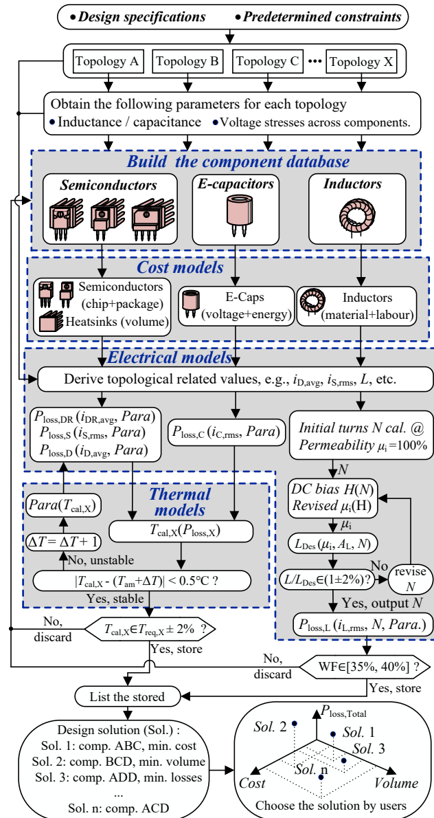
Fig. 9. Design procedure for the topology benchmarking. Initially, the procedure calculates the stable junction/hot-spot temperature of each component and the winding factor of each core in the component database by the electro-thermal loop and the permeability-related turn calculation loop (details in Section III-F). Then, it lists the stored (requirement-fulfilled) components or component combinations (including heatsinks) with cost, volume, and power loss for users to select them based on their design priorities.
