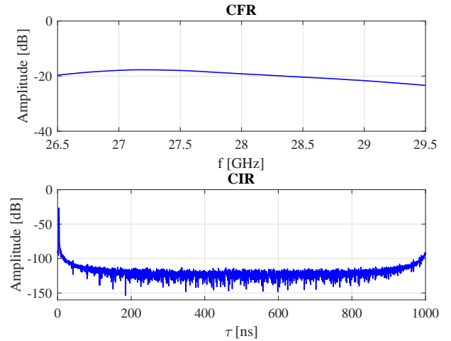
Fig. 7. Measured CFR ( S_{43} with frequency range from 26.5 to 29.5 GHz) and CIR of the channel between SGH port and AiP port.
