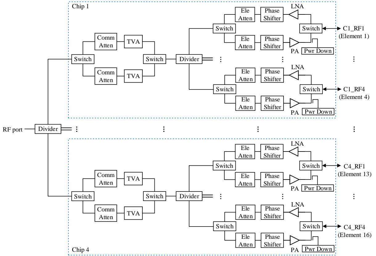
Fig. 2. Block diagram of the AiP.
