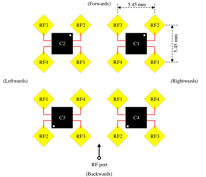
Fig. 3. Antenna view of the AiP.
