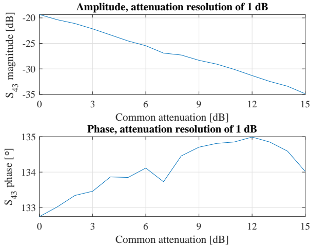
Fig. 12. Complex S_{43} as a function of the common attenuation in the “all-on” mode.
