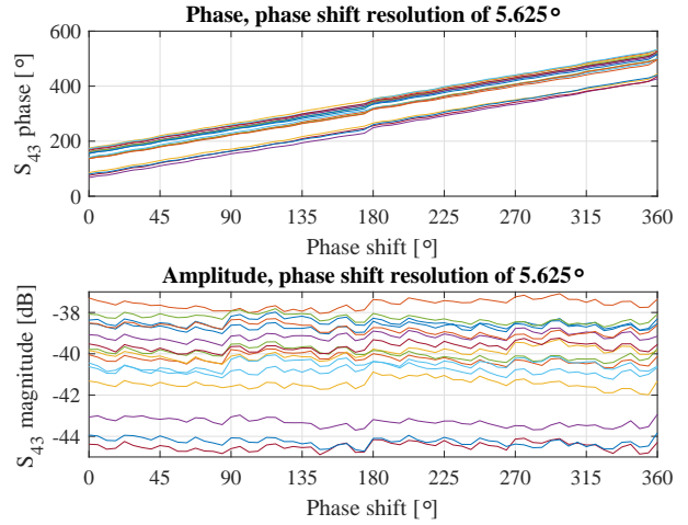
Fig. 11. Complex S_{43} as a function of the phase shift in the “on-off” mode. 16 curves stands for 16 elements.
