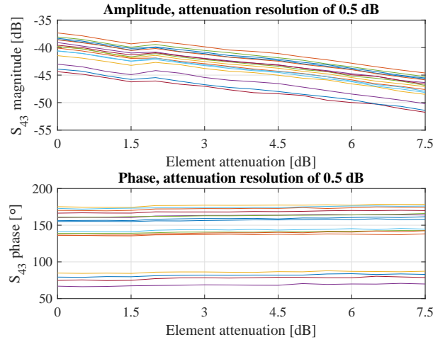
Fig. 10. Complex S_{43} as a function of the element attenuation in the “on-off” mode. 16 curves stands for 16 elements.
