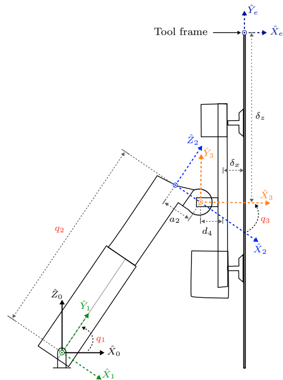
Fig. 2. Sketch of the Wallmo robot along with local joint frames. The generalized coordinates used in the installation procedure ( q_1, q_2, q_3 ) are marked by red text color. The DH parameters can be found in the Appendix. Source Sloth and Pedersen (2017)
