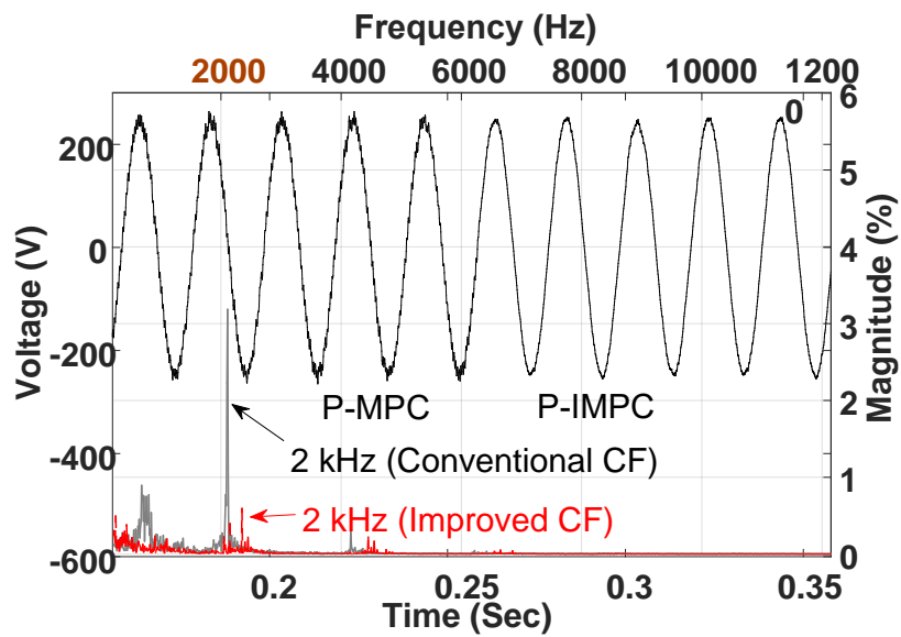
Figure 12. Obtained experimental voltage and spectrum results using the conventional and improved CFs. F_{sw} = 2 \text{ kHz} , C_f = 60 \mu\text{F} , L_f = 5 \text{ mH} .
