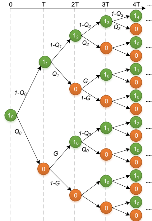
Fig. 3. Tree diagram of a system considering non-exponential failure rate.
