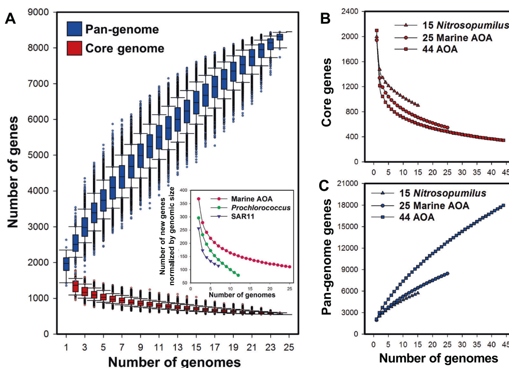
Fig. 2 AOA core genome and pan-genome analyses. a Box-and-whisker plots of core and pan-genome sizes of 25 marine AOA species. The number of genes is plotted as a function of the number of n strains sequentially added. For n genomes selected out of 25, there are 25!/[(n-1)!(25-n)!] possible combinations from which to calculate core and pan-genomes. Each possible combination is plotted as a red and a blue dot for core genome and pan-genome analysis, respectively. To compare the pan-genome openness of marine AOA species with
