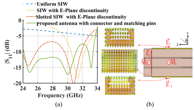
Fig. 2. (a) The reflection coefficient of the proposed single element and comparison with other configurations. (b) Equivalent magnetic currents of the electric field on the slots and open end of the SIW at 29 GHz.
