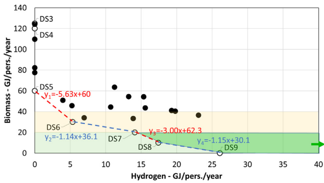
Fig. 4. The 9 generic design strategies represented by open white dots compared to the 16 scenarios represented by black dots. Equations for the red trend lines are shown in red and the equations for the blue trend lines are shown in blue. The red lines include a change in the degree of electrification, whereas the blue lines represent a fixed degree of electrification. Note that the exact numbers for the generic design strategies are plotted, not the rounded numbers from the illustrations. The light green area indicates the sustainable technical potential of biomass on a global scale, the yellow area indicates the Danish biomass potential, and the more intense green area and the arrow indicates the feasible and sustainable operating point for an energy system. The more intense green area stretching to the right as indicated by the arrow thus represents the technically feasible and environmentally sustainable ‘solution space’ for the transition to a fully renewable energy system.
