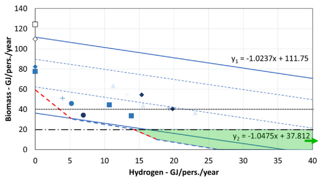
Fig. 5. The relation between biomass and hydrogen for all 16 scenarios and their degree of electrification. The thick blue lines, y_1 and y_2 , are based on the simplistic system model where the degree of electrification is completely fixed. The correlation equations related to each line respectively is placed just above the line. New on this Figure is also the two thin blue punctured lines indicating not further specified degrees of electrification between y_1 and y_2 . The Danish and global biomass potential is now shown respectively as a horizontal black dotted line and a horizontal black dash-dot-dash line. The DEA scenarios are represented by squares, the SDU scenarios by diamonds, the CEESA scenarios by triangles, the Energinet scenarios by dots, and the IDA scenarios by pluses. The shading of the scenarios represents the degree of electrification i.e. no shade (white) is an electrification of less than 5 GJ/pers./year of electricity for heat and transport, light shade between 5 and 10 GJ/pers./year of electricity for heat and transport, medium shade between 10 and 15 GJ/pers./year of electricity for heat and transport, and dark shade more than 15 GJ/pers./year of electricity for heat and transport.
