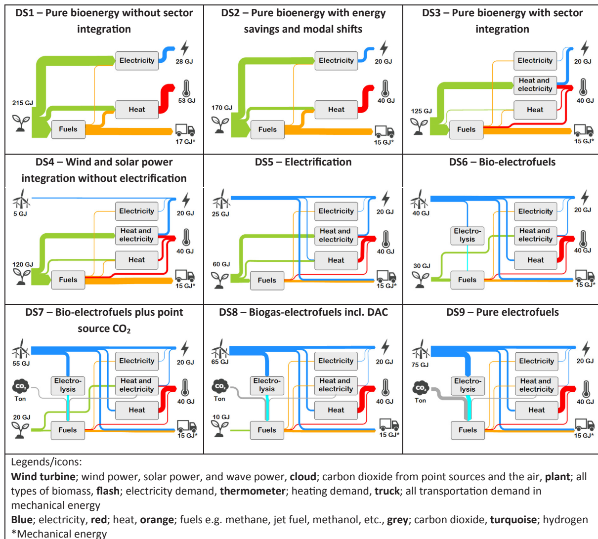
Fig. 2. Generic design strategies. The amounts are expressed in GJ per person per year. Only GJ is shown to improve the readability of the Sankey diagrams. For an explanation of each generic design strategy, see text below.
