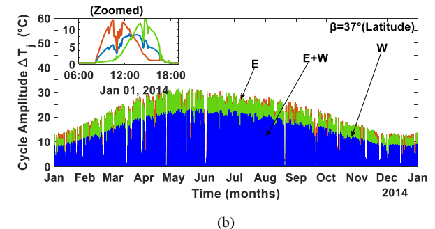
Fig. 19. Thermal loading of a single IGBT device in the PV inverter for yearly mission profile data with different Orientation: East, West, E+W split: (a) Mean junction temperature T_{jm} and (b) Cycle amplitude of the junction temperature variation \Delta T_j .
