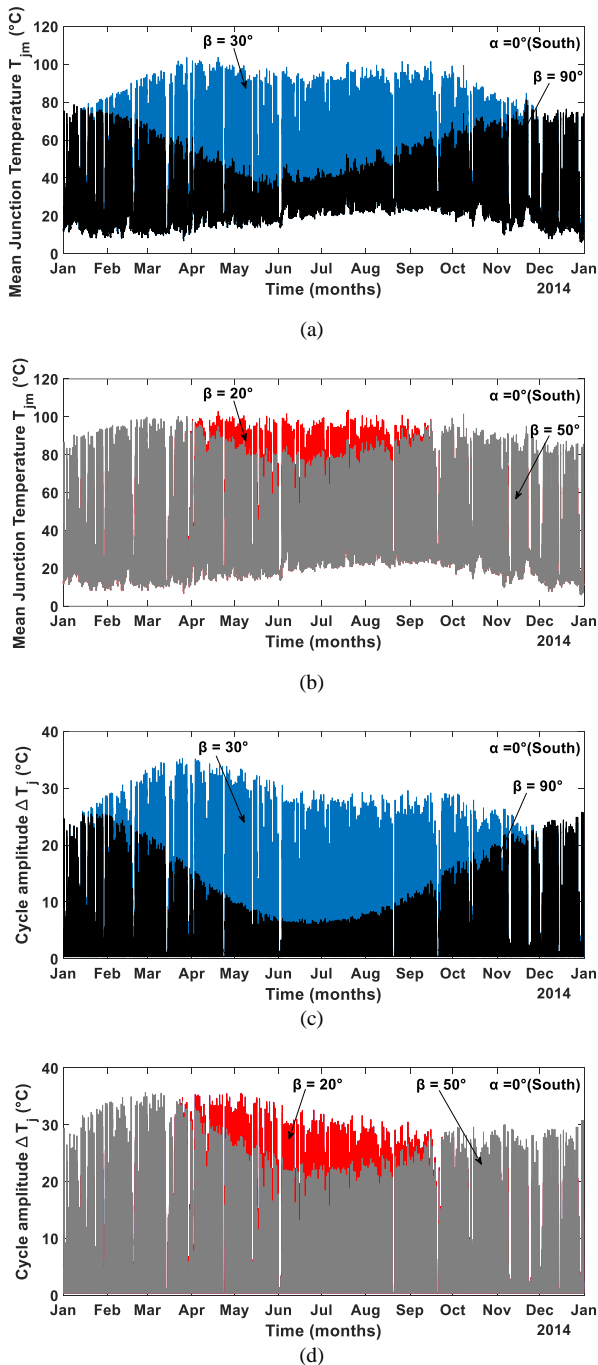
Fig. 9. Thermal loading of a single IGBT device in the PV inverter for yearly mission profile data with different tilts angles \beta : (a,b) Mean junction temperature T_{jm} and (c,d) Cycle amplitude of the junction temperature variation \Delta T_j .
