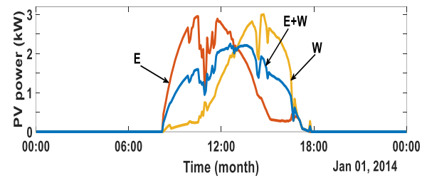
Fig. 18. Available power from PV panels in 1 day for different orientation of PV panels: East, West, E+W split.
