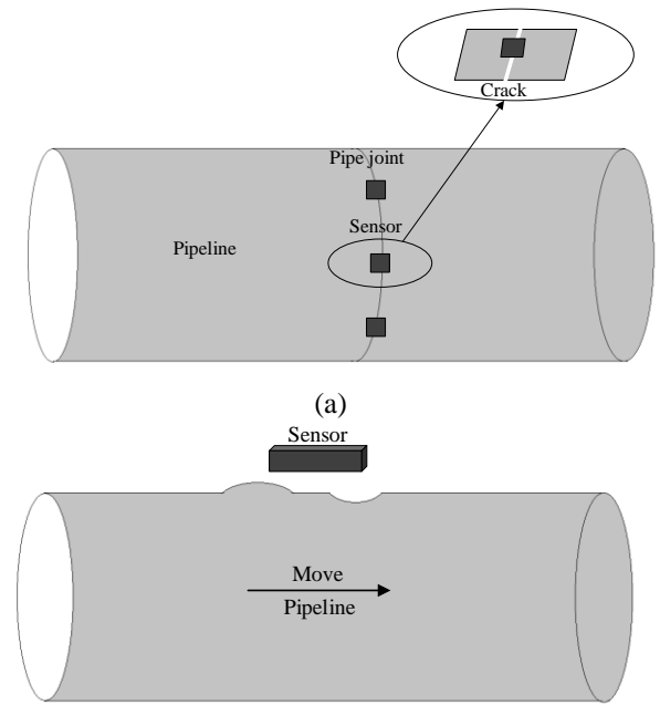
Fig. 8 Two kinds of application (a) permanent installation, (b) scanning application
