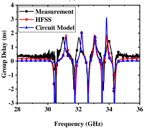
Fig. 2. Measurement, simulation and circuit model results of the multiband sensor.
