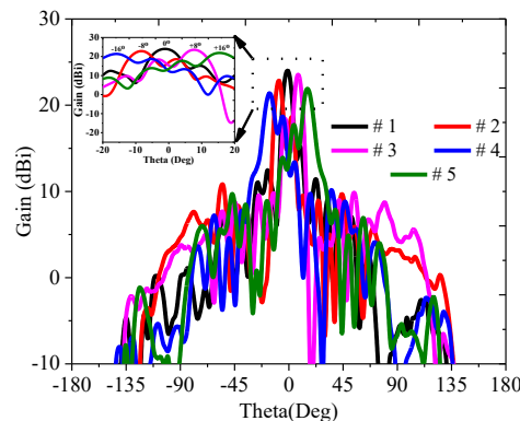
Fig. 22. The measured gains of the beam-steerable TA antenna with five beams at 27.2 GHz.
