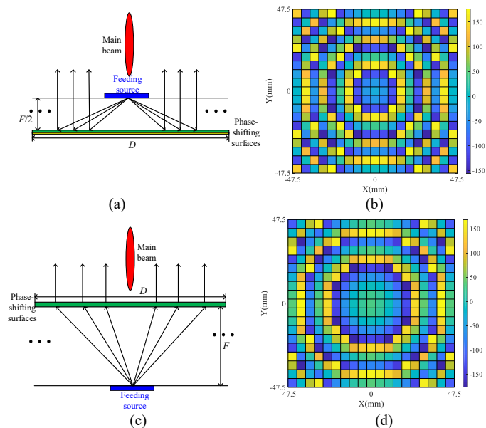
Fig. 9. (a). The schematic diagram of the RA antenna for reference. (b). The corresponding phase distributions. (c). The schematic diagram of the TA antenna for reference. (d). The corresponding phase distributions.
