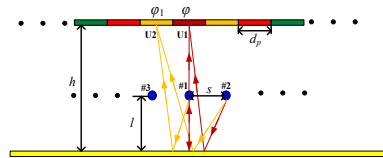
Fig. 16. The simplified schematic diagram for the beam-steerable TA antenna.
