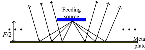
Fig. 3. The configuration of the exact feeding source.
