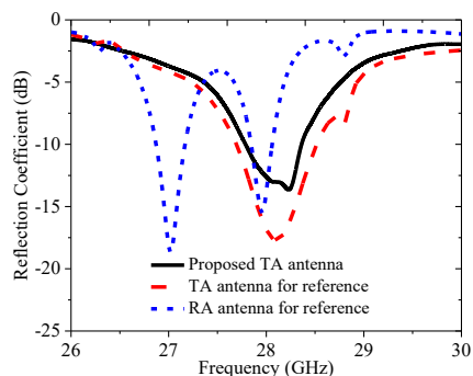
Fig. 10. The reflection coefficients of the three antennas.
