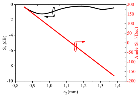
Fig. 6. The transmission phase and transmission amplitude of the unit cell with different values of r_2 . ( h = 0.305 mm, H = 2.5 mm, r_4 = 2.25 mm, r_3 = 1.75 mm, r_2 - r_1 = 0.5 mm)
