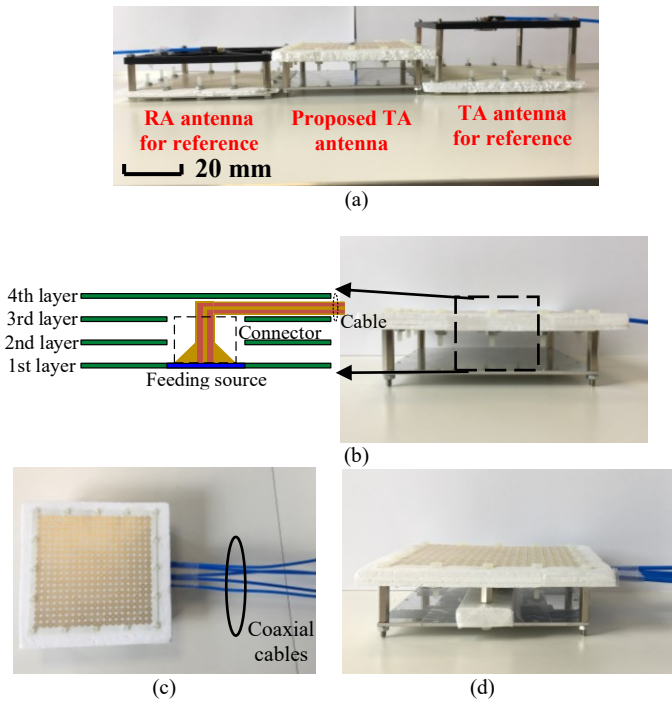
Fig. 17. The photographs of the proposed TA antenna, the RA antenna for reference, the TA antenna for reference, and the beam-steerable TA antenna with five beams. (a). Side view of the RA antenna for reference, the proposed TA antenna, and the TA antenna for reference. (b). Side view of the proposed TA antenna. (c). Front view of the beam-steerable TA antenna with five beams. (d). Side view of the beam-steerable TA antenna.
