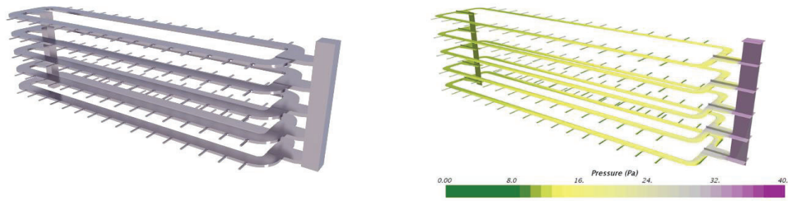
Figure 9. CFD-design calculations of a low pressure ring ductwork system
