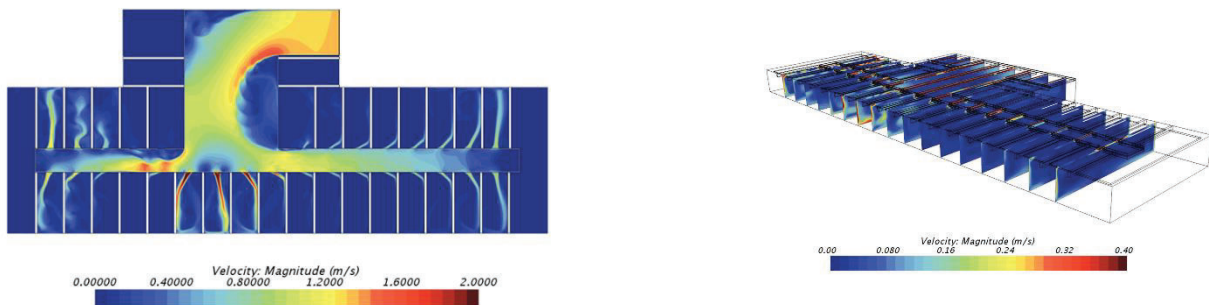
Figure 5. Results of CFD feasibility analyses of air flows
