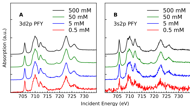
FIG. 1. Comparison of (a) Fe 3d2p PFY-XAS and (b) Fe 3s2p PFY-XAS measurements for all concentrations of aqueous \text{K}_3[\text{Fe}(\text{CN})_6] . Spectra have been scaled and vertically offset for clarity. Spectra for 500 mM, 50 mM, and 5 mM concentrations were acquired in 5 h each, while the 0.5 mM spectrum took 15 h of measurement. The 3d2p signal has six times greater intensity than the 3s2p signal.
