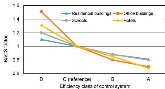
Fig. 1. BACS factor (reduction ratio) for efficiency classes effect on energy use for room conditioning (heating or cooling) for residential buildings, office buildings, hotels and schools, class C is defined as the reference configuration, data from EN 15232 [11].
