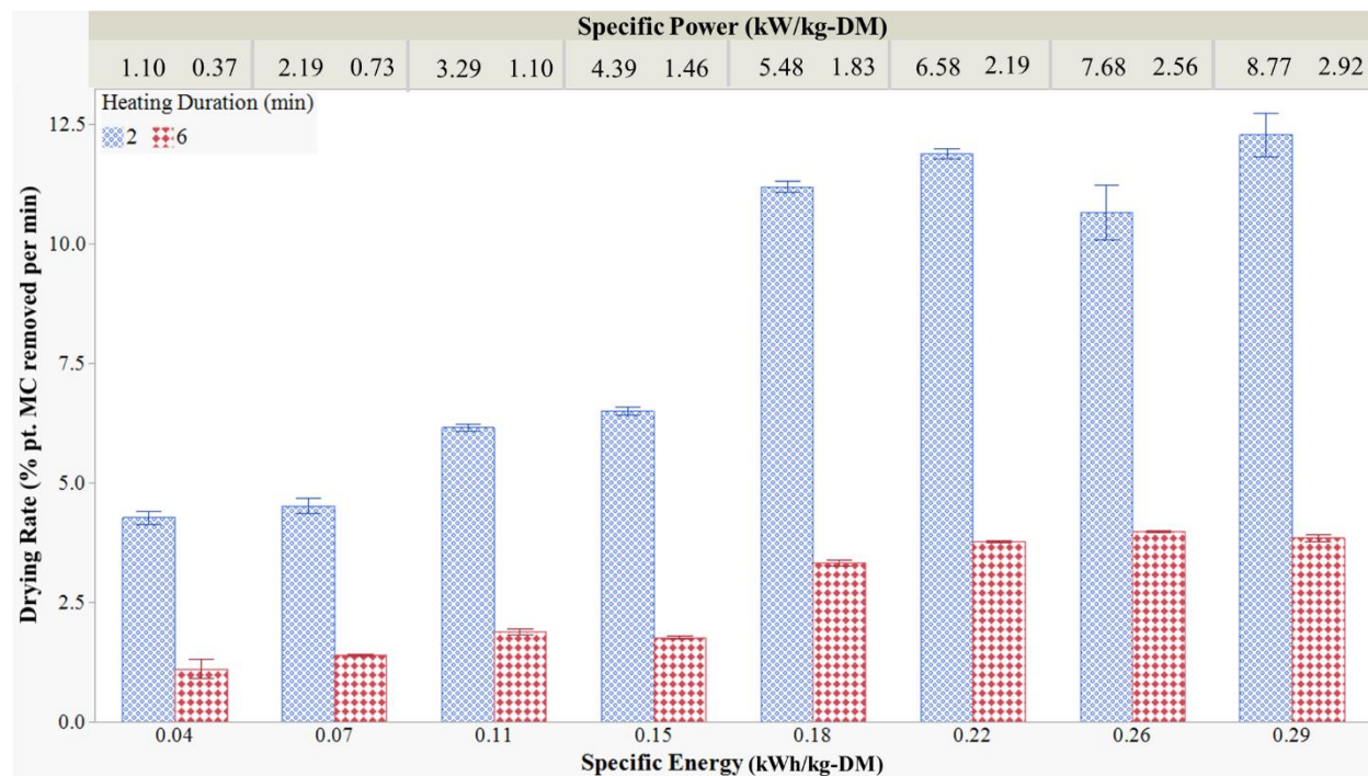
Figure 3.3: Effect of microwave specific power on the drying rate of parboiled rough rice dried using a microwave at 915 MHz frequency; % pt indicates percentage points; MC indicates moisture content in dry basis; kg-DM indicates kg of dry matter (DM).
