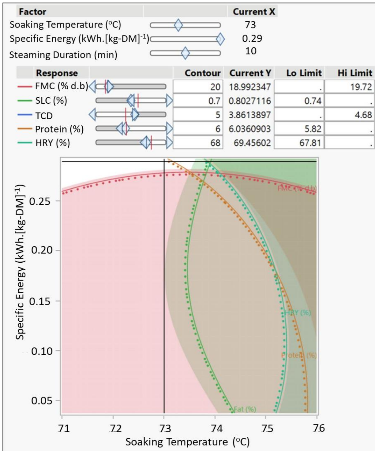
Figure 2.5: Contour Profiler for the head rice yield (HRV), protein content, surface lipid content (SLC), final moisture content (FMC) and total color difference (TCD) responses with parameter settings soaking temperature, MW specific energy and steaming duration; kg-DM indicates kg of dry matter
