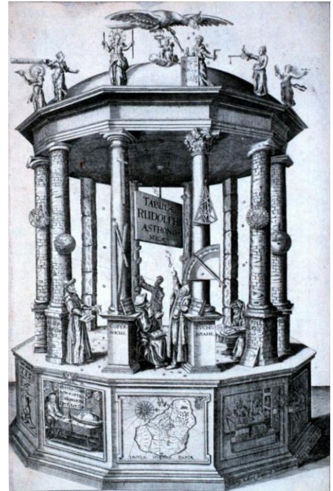
Figure 4: Movement into the "New" Astronomy
