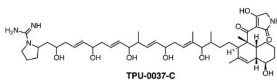
Fig. 4. Structures of the identified antibiotic compounds from isolated actinomycetes strains in Switzerland, namely azalomycin F 4a 2-ethylpentyl ester, [18,19] TPU-0037-C, [20,21] bottromycin A2, [22] echinomycin, [23] milbemycin- \alpha , [24] dihydropicromycin. [25] The structure of bafilomycin A1 is shown in the publication of Yu et al. [26] and a proposed derivative of the compound is published in the patent CN104817547 (B).
