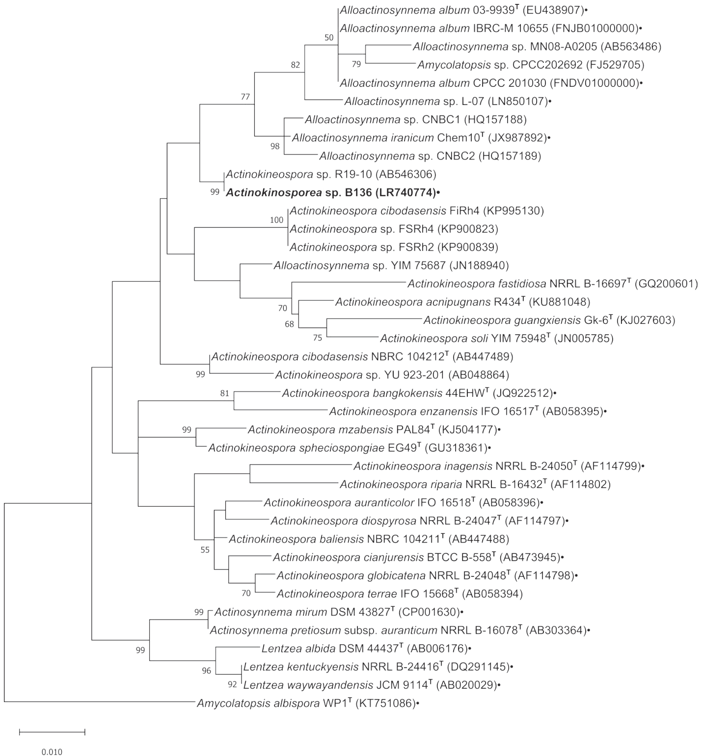
Fig. 5. Phylogenetic position of Actinokineospora B136.1 with its closely related taxa based on 16S rRNA sequences. The tree with the highest log likelihood (-5946.57) is shown. The percentage of trees out of 1000 replications in which the associated taxa clustered together is shown next to the branches when above 50%, and the scale bar represents the percentage of substitutions per site. Initial tree(s) for the heuristic search were obtained automatically by applying Neighbor-Joining and BioNJ algorithms to a matrix of pairwise distances estimated using the Maximum Composite Likelihood (MCL) approach, and then selecting the topology with superior log likelihood value. The type strain of the species is highlighted with a bold superscript T after the strain information; accession numbers are provided between brackets after the strain information and genome sequenced strains are highlighted with a dot after the accession number. Amycolatopsis albispora WP1 T was used as outgroup.
