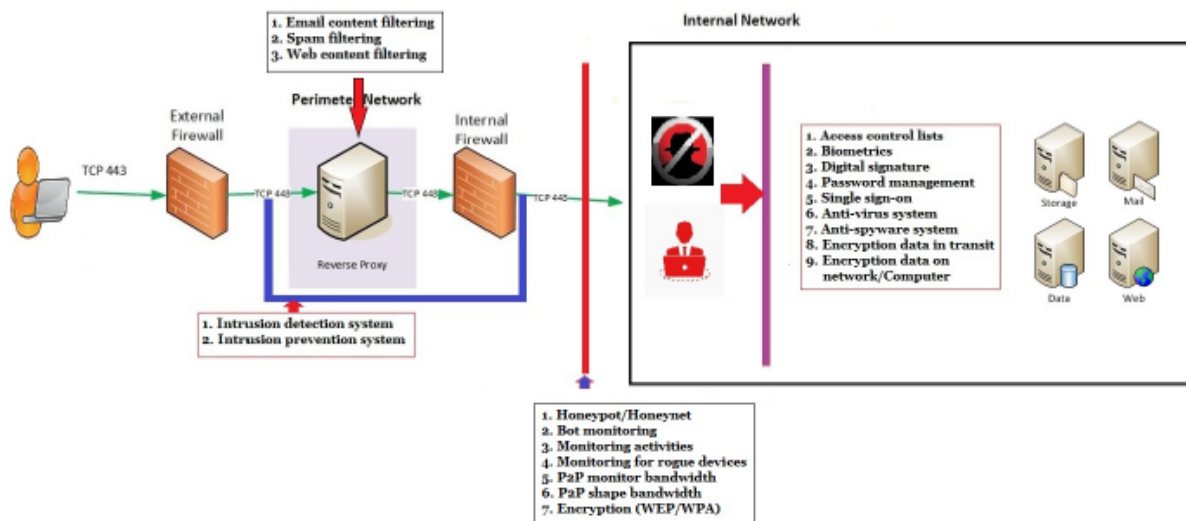
Figure 1. Diagram of Cybersecurity System Structure
