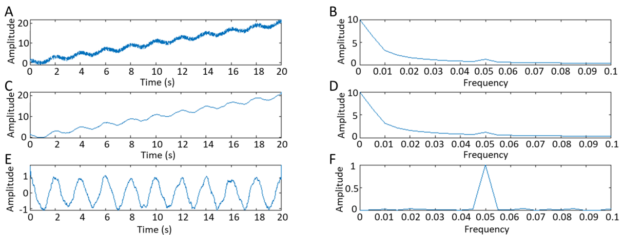
Figure 2.4: Data preparation steps for FFT analysis. (A) A raw noisy signal with a linear trend and (B) corresponding FFT output for that signal. (C) The signal after applying a 10-point smoothing filter and (D) corresponding FFT output. (E) The signal after being linearly detrended and (F) corresponding FFT output which shows a clear distinct peak with a smaller scale to clearly see the peak.
