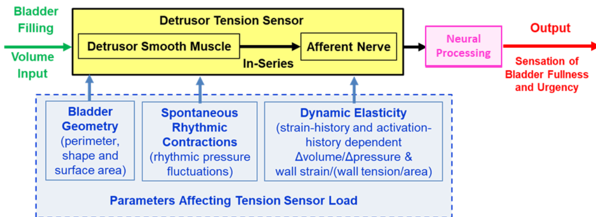
Figure 3.1: Detrusor tension sensor model. Model showing detrusor as a tension sensor and the parameters affecting the load applied to this tension sensor.
