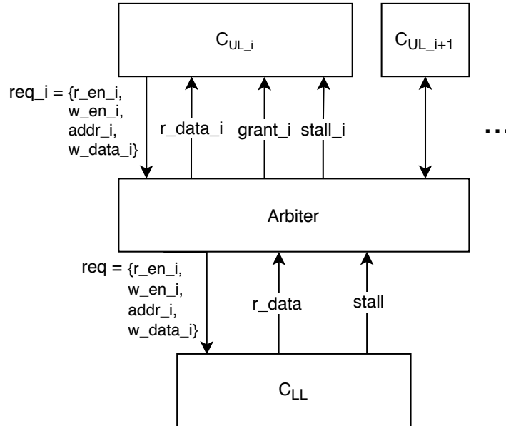
Figure 2.13: Arbiter interface.
