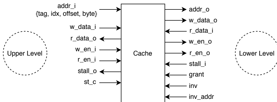
Figure 2.15: Cache interface.
