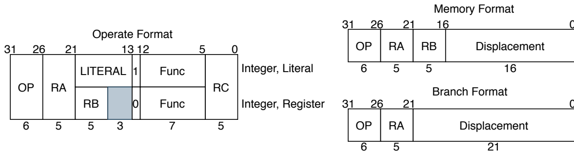
Figure 2.1: Instruction formats in Alpha architecture [34].
