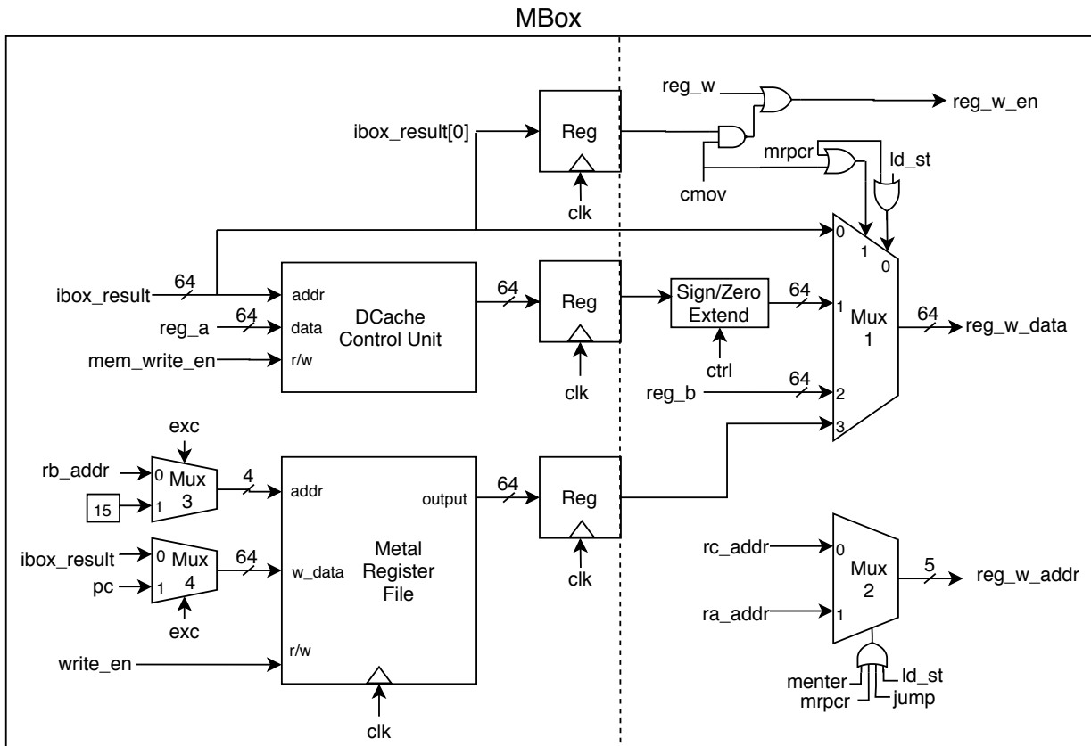
Figure 2.11: MBox block diagram.
